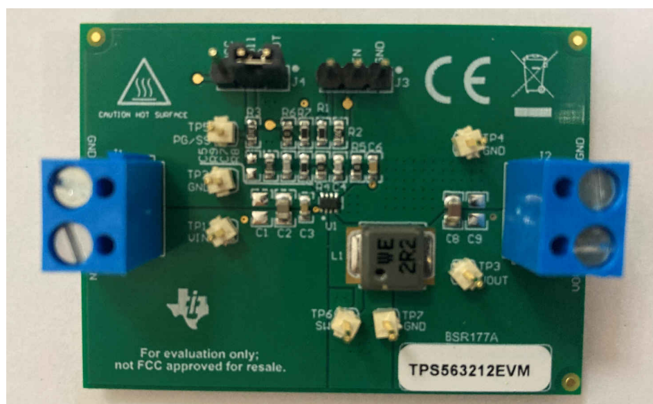
Figure 5-4. TPS563212EVM Board (Top View)
