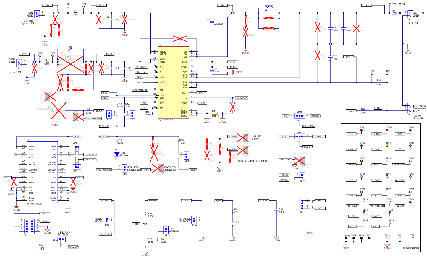
Figure 4-1. BQ25630EVM Schematic
