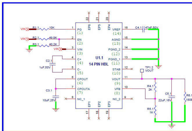
Figure 2-1. Bias Diagram Used in TID Exposure
