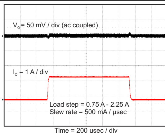
Figure 8-26. Tps563200 Transient Response
