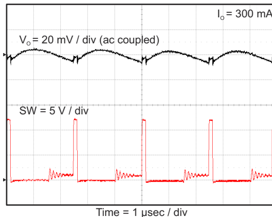
Figure 8-24. Tps563200 Output Voltage Ripple
