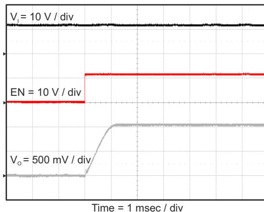
Figure 8-28. Tps563200 Start-up Relative to EN
