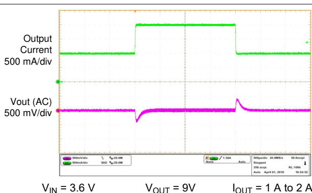
Figure 9-7. Load Transient
