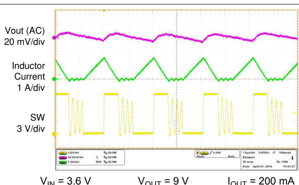
Figure 9-3. Switching Waveforms in DCM
