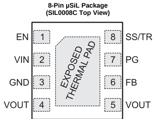
Pin Functions
