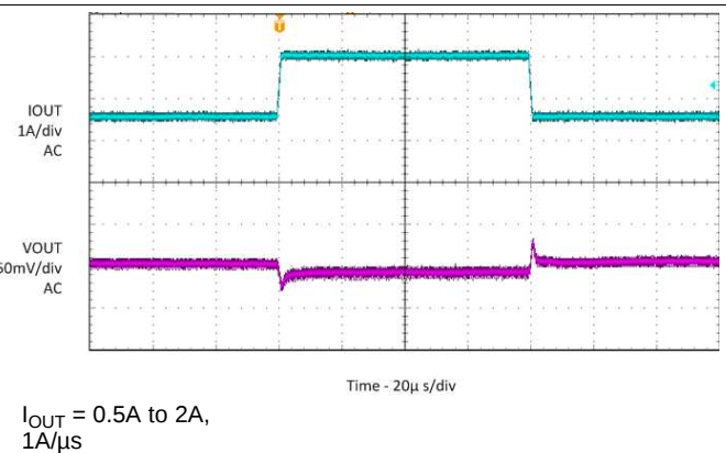
Figure 27. Load Transient
