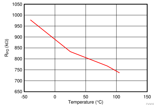
Figure 7-4. Quick Output Discharge (QOD)
