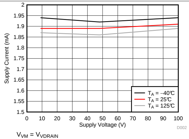
Figure 3. VDDRAIN Supply Current Over Supply Voltage
