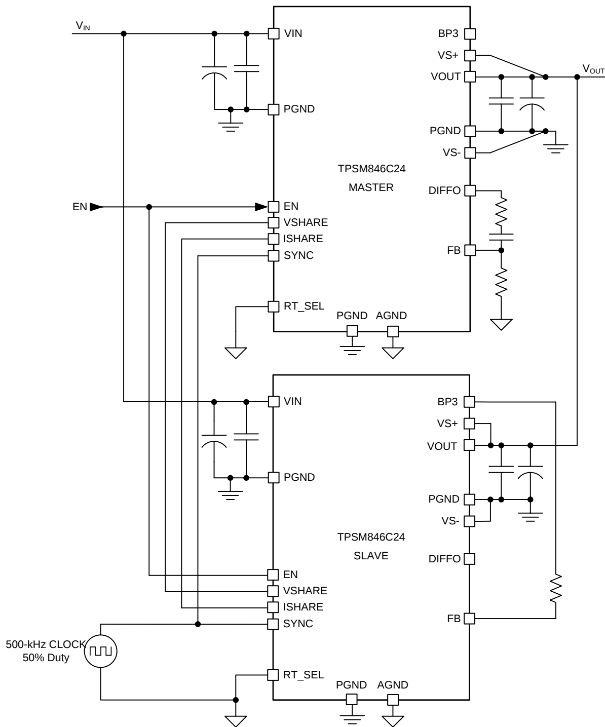
Figure 16. TPSM846C24 Parallel
