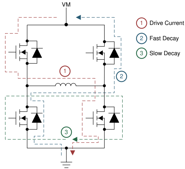
Figure 7-12. Decay Modes
