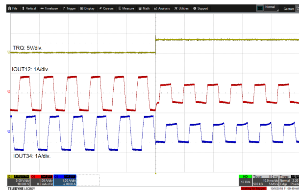
Figure 8-12. Torque Pin Functionality for Current Scaling
