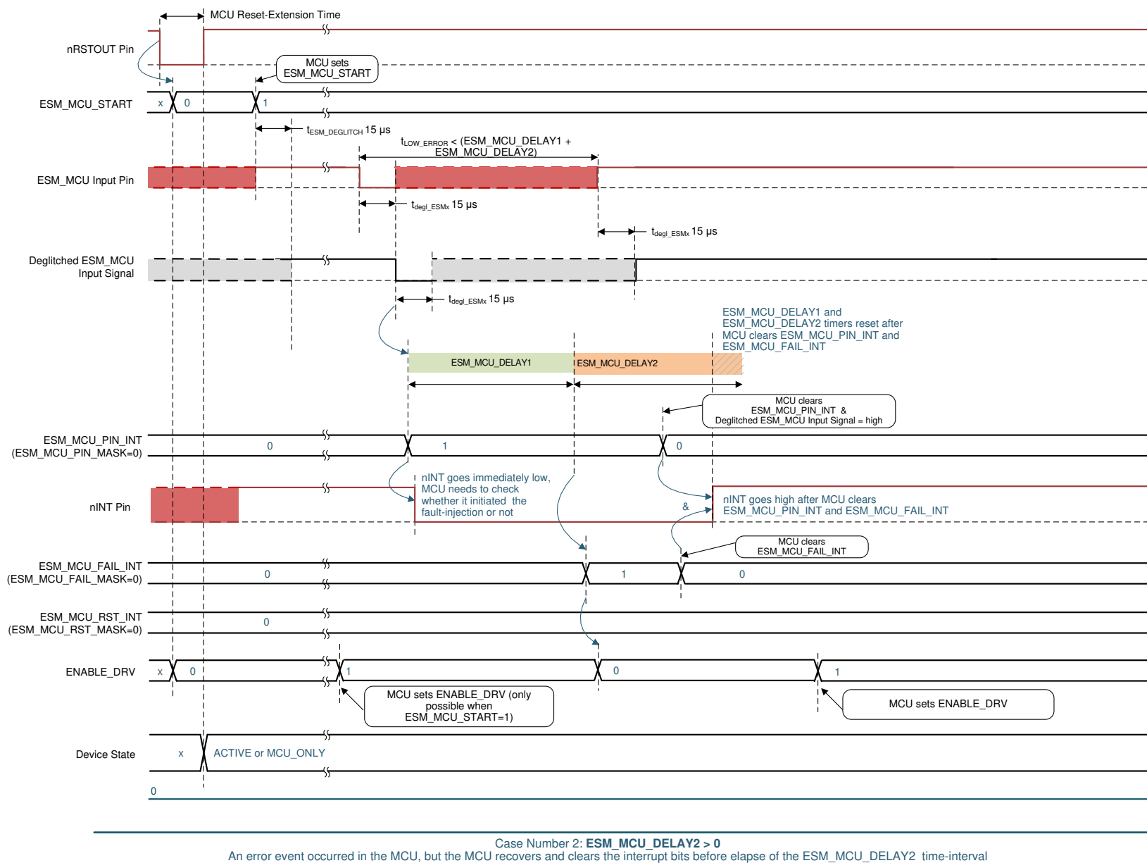
Figure 8-30. Example Waveform for ESM in Level Mode – Case Number 2: Delay-2 Not Set To 0 and \text{ESM\_MCU\_ENDRV}=1 , \text{ESM\_MCU} Signal Recovers Elapse of Delay-2 Time-Interval
