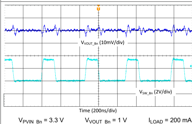
Figure 9-32. Buck Output Ripple - 4-Phase, Fsw = 2.2 MHz, Forced-PWM Mode
