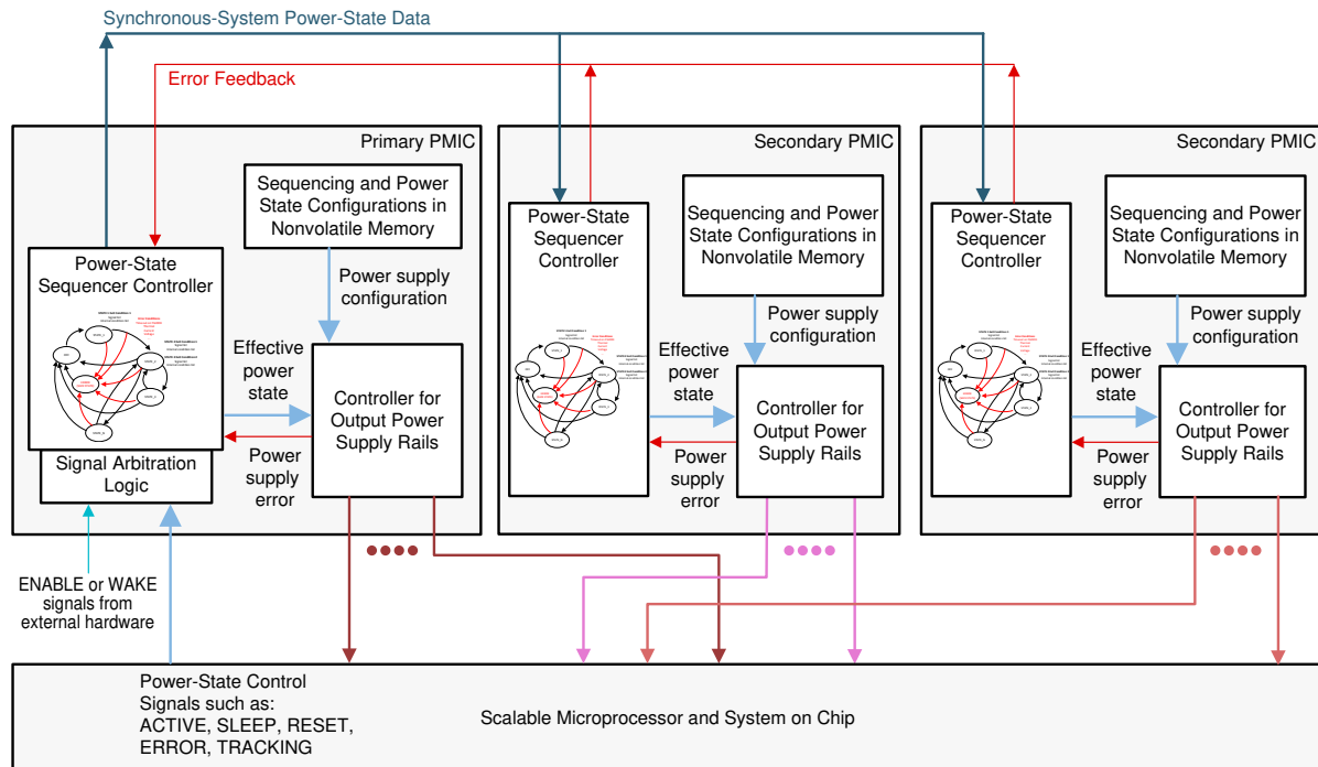
Figure 8-46. Multi-PMIC Power State Synchronization Block Diagram
