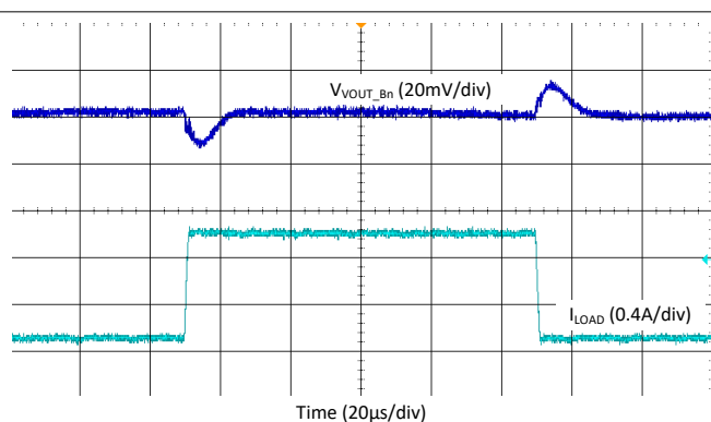
Figure 9-54. Buck Load Step Transient - Buck5, 2.2 MHz, Auto Mode
