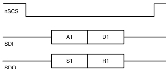
Figure 7-23. SPI Transaction Between MCU and the device
