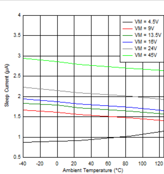
Figure 6-2. Sleep Current over Temperature
