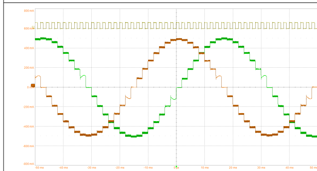
Figure 8-5. 1/8 Microstepping With Mixed30-Mixed30 Decay
