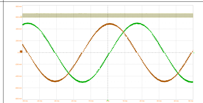
Figure 8-10. 1/32 Microstepping With smart tune Dynamic Decay
