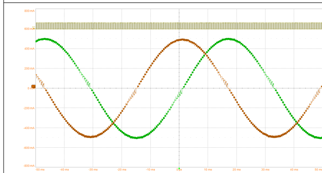
Figure 8-9. 1/32 Microstepping With smart tune Ripple Control Decay
