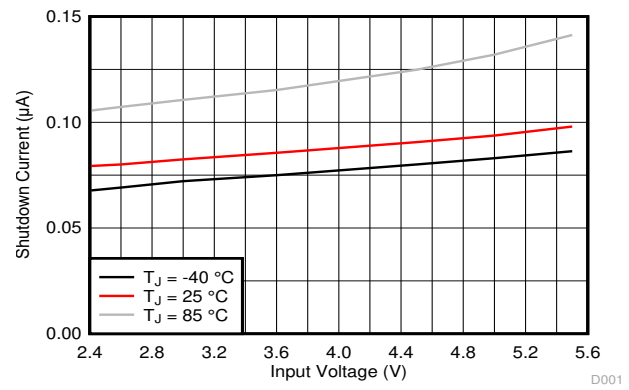
Figure 7-4. Shutdown Current
