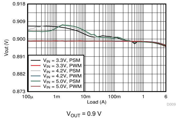
Figure 9-5. Load Regulation
