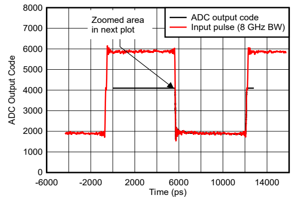
Figure 5-146. Pulse Overdrive Recovery
