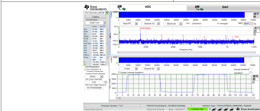
Figure 7-12. 200-MHz, Sine-Wave (Channel A) Frequency Domain (FFT) and 40-MHz, Square-Wave (Channel B) Time Domain for 5-GSPS, Single-Channel Oscilloscope
