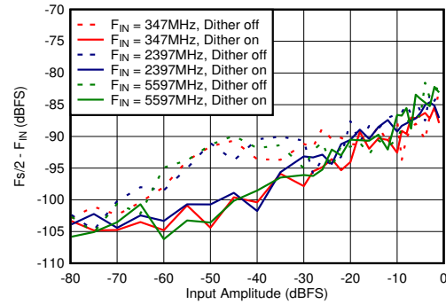
Figure 5-80. Dual Channel Mode: F_s/2 - F_{IN} vs Input Amplitude and Dither
