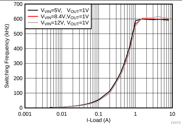
Figure 20. F_{SW} Load Regulation, Eco-mode, F_{SW} = 600\text{ kHz}
