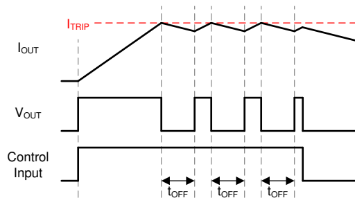
Figure 7-3. Off-Time Current-Regulation
