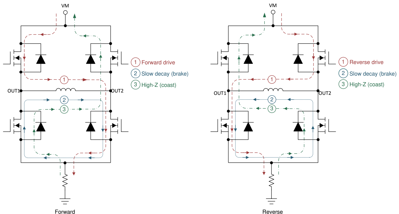
Figure 7-1. H-Bridge States
