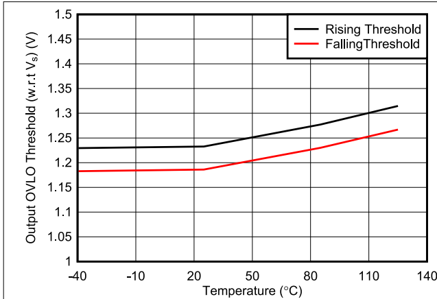
Figure 7-13. OUT OVLO Thresholds (w.r.t Vs) vs Temperature for TPS26612
