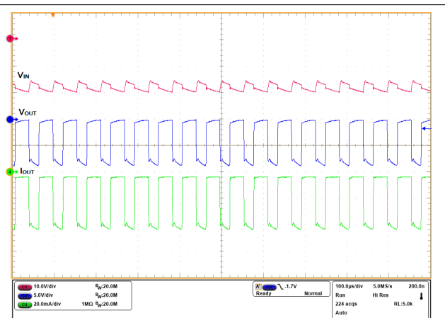
Figure 8-17. Thermal Protection During Loop Testing for I_{LOOP} < 0
