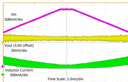
Figure 8-9. Line Transient
