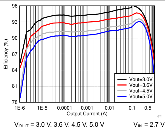
Figure 6-5. Efficiency with Different Outputs in Boost Operation
