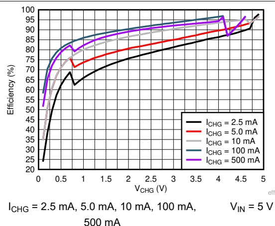
Figure 6-6. 5-V Input Efficiency with Different Charging current in Buck Operation
