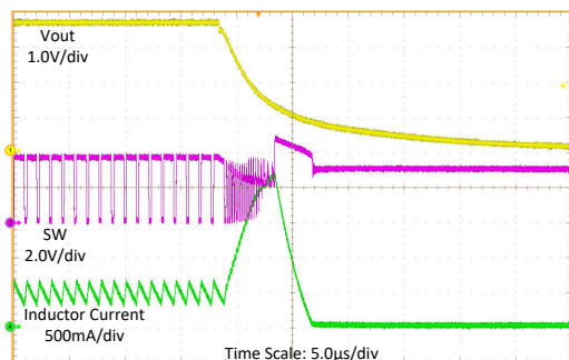
Figure 8-10. Load Sweep
