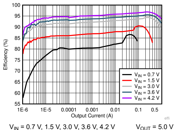
Figure 6-1. 5.0-V V_{OUT} Efficiency with Different Inputs in Boost Operation
