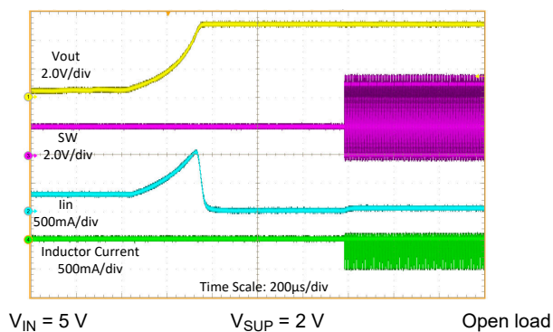
Figure 8-23. Output Short Protection (Recover)
