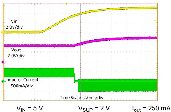
Figure 8-21. V_{IN} Power On and Charging Automatically
