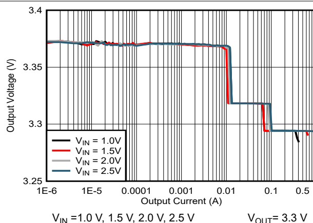
Figure 6-4. 3.3-V Load Regulation in Boost Operation
