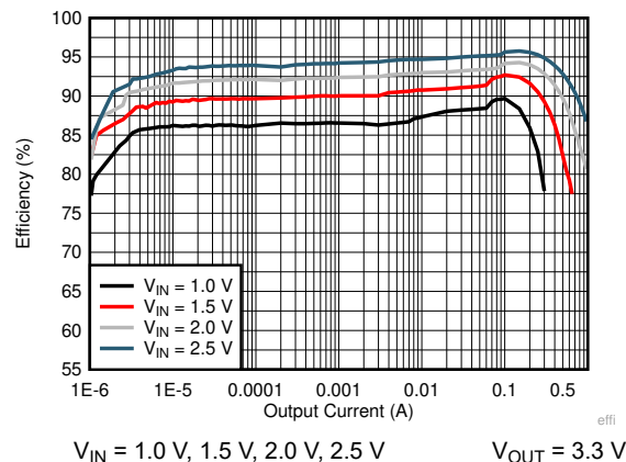
Figure 6-2. 3.3-V V_{OUT} Efficiency with Different Inputs in Boost Operation
