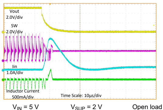
Figure 8-22. Output Short Protection (Entry)
