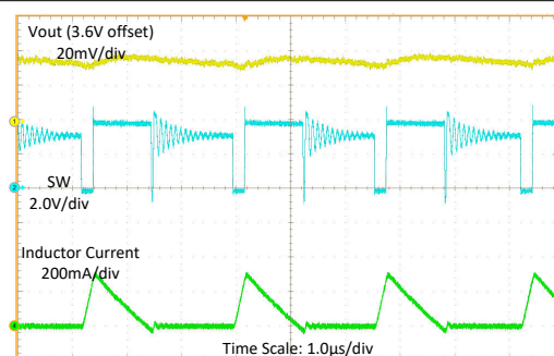
Figure 8-3. Switching Waveform at Medium Load
