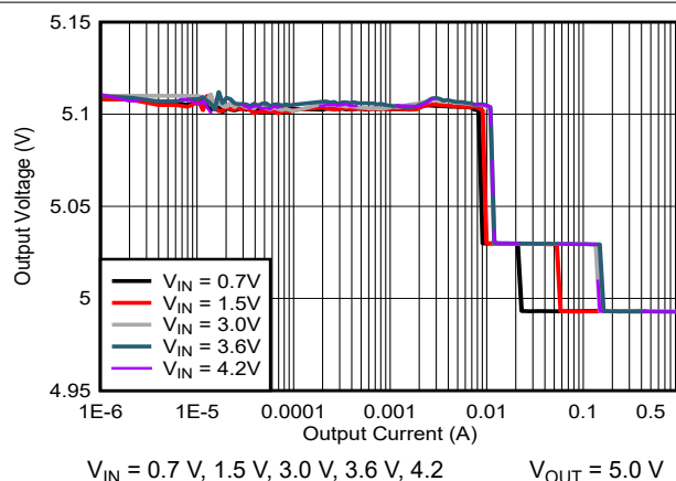
Figure 6-3. 5.0-V Load Regulation in Boost Operation
