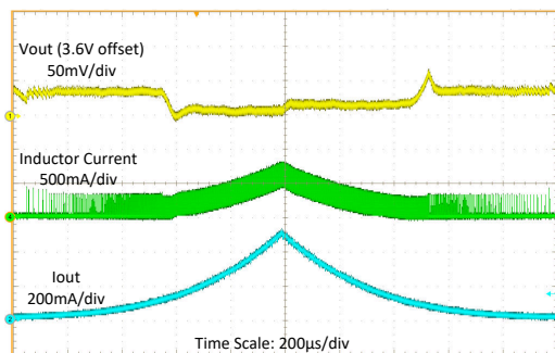
Figure 8-8. Load Transient at Boost Mode
