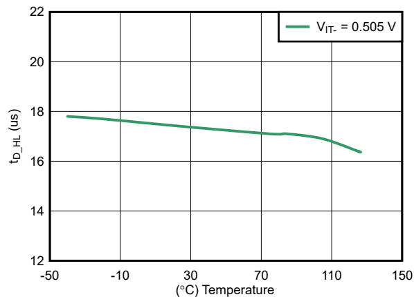
Figure 6-9. SENSE Delay ( t_{D\_HL} ) vs Temperature
