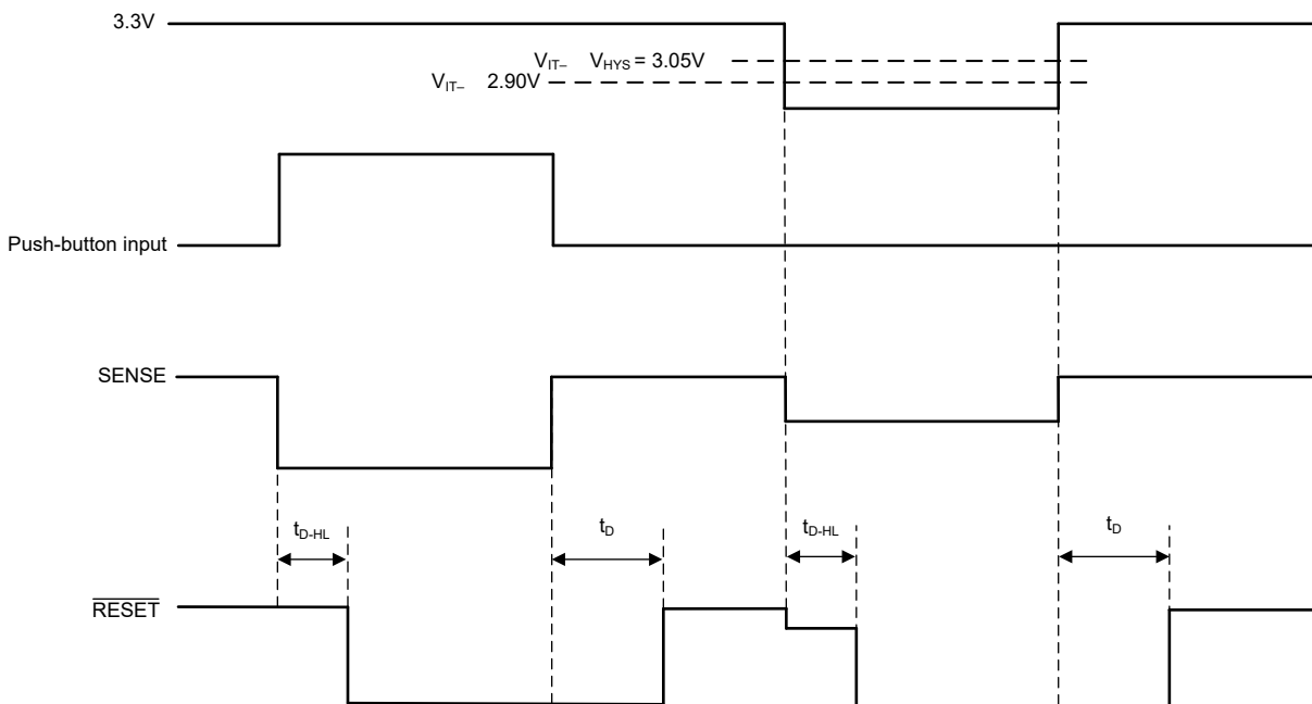
Figure 8-2. Design 1 Timing Diagram
