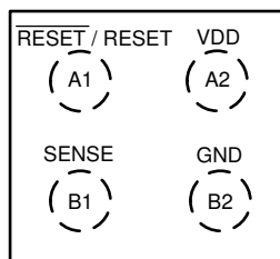
Figure 5-1. YBH 4-Pin DSBGA Package (TLV841S) Top View
