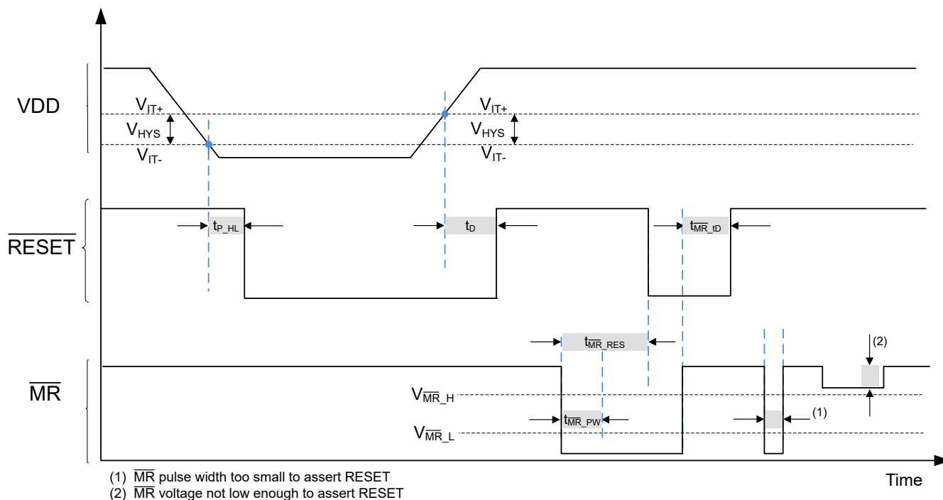
Figure 6-3. Timing Diagram for TLV841CxxL (CT) Active Low Output [Open-Drain and Push-Pull Output Topology]
