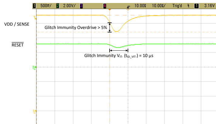
Figure 8-5. TLV841EVM SENSE Pin Glitch Immunity ( t_{GL\_VIT-} )
