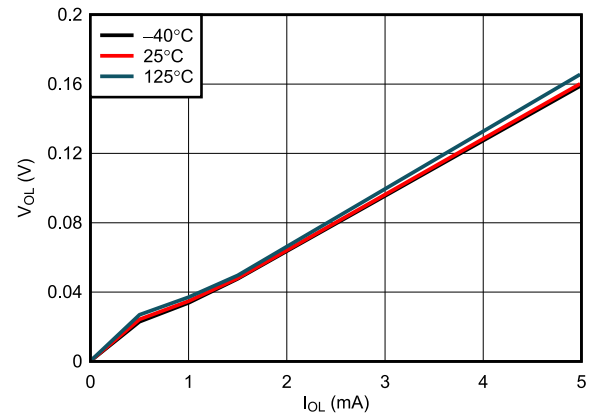
Figure 6-10. V_{OL} vs I_{OL}
