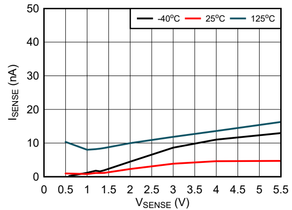
Figure 6-6. SENSE Current vs V_{\text{SENSE}}
