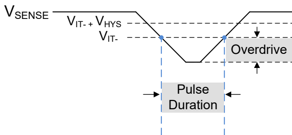
Figure 7-4. Overdrive vs Pulse Duration
