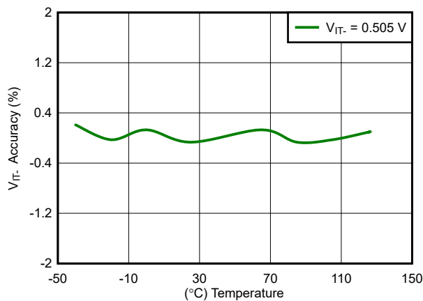
Figure 6-7. V_{\text{IT-}} Accuracy vs Temperature
