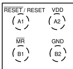
Figure 5-3. YBH 4-Pin DSBGA Package (TLV841M) Top View
