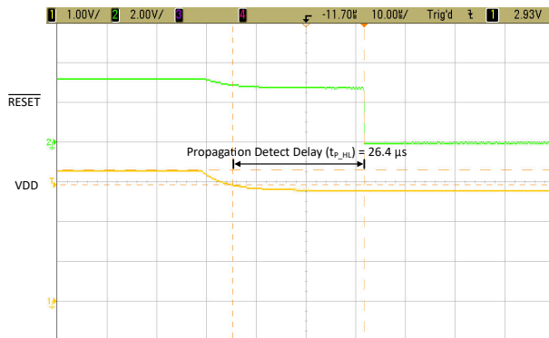
Figure 8-3. TLV841EVM Propagation Delay Time Delay ( t_{D\_HL} )
