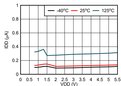
Typical Supply Current
