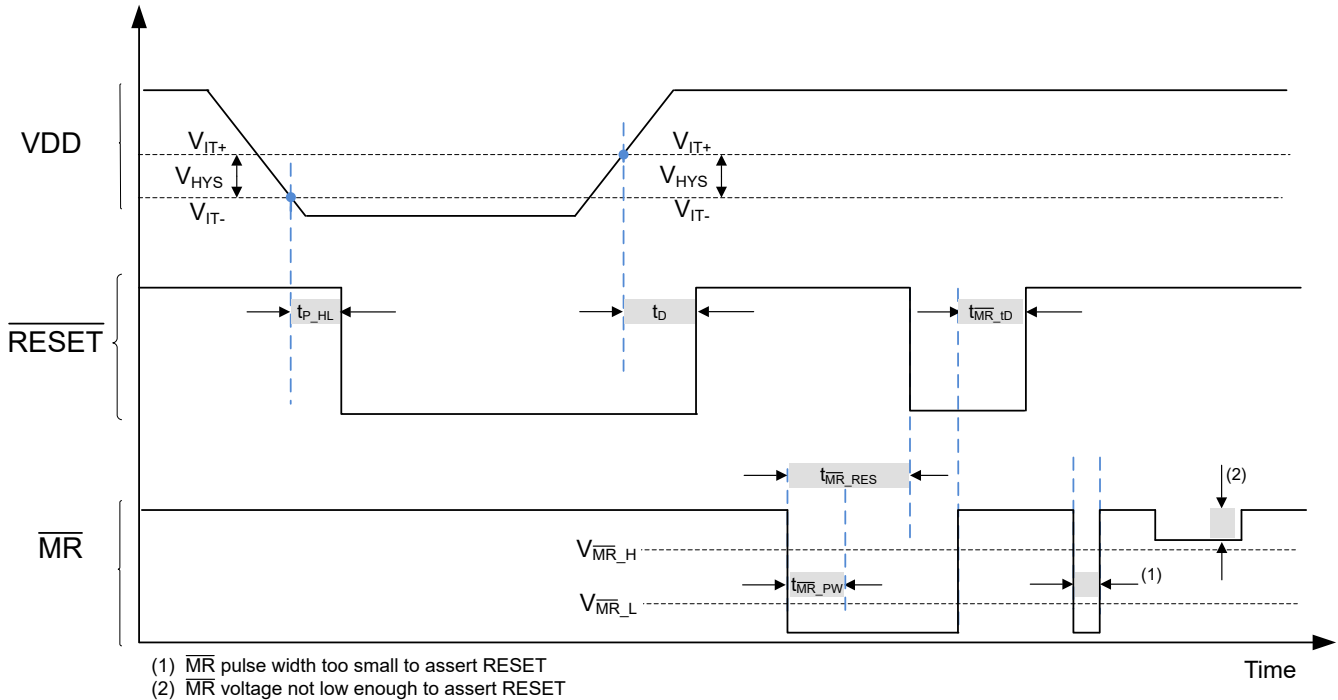
Figure 7-6. Timing Diagram \overline{\text{MR}} and \overline{\text{RESET}} (TLV841M)
