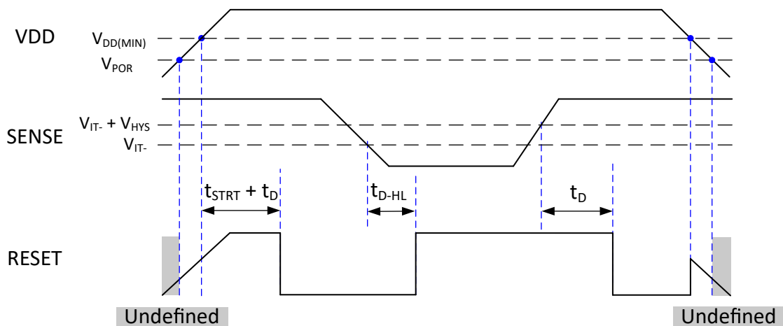
Figure 6-1. Timing Diagram for TLV841SxxL (SENSE) Active Low Output [Open-Drain and Push-Pull Output Topology]
