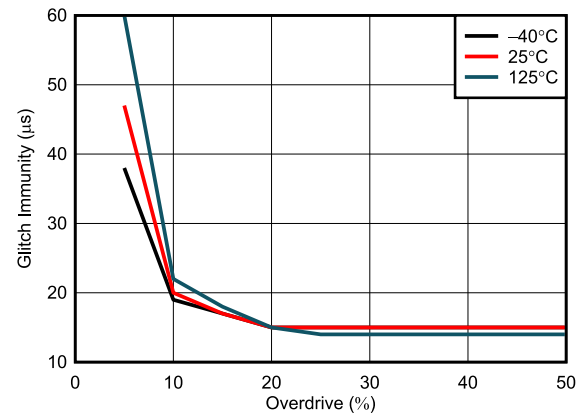
Figure 6-8. SENSE Glitch Immunity ( V_{\text{IT-}} ) vs Overdrive
