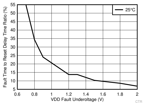
Figure 7-5. C_{CT\_EXT} Discharge Time During Fault Condition ( C_{CT\_EXT} = 1\mu F )
