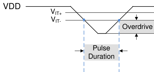
Figure 7-2. Overdrive vs Pulse Duration
