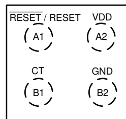
Figure 5-2. YBH 4-Pin DSBGA Package (TLV841C) Top View
