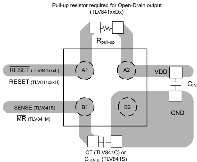
Figure 8-6. TLV841 Recommended Layout
