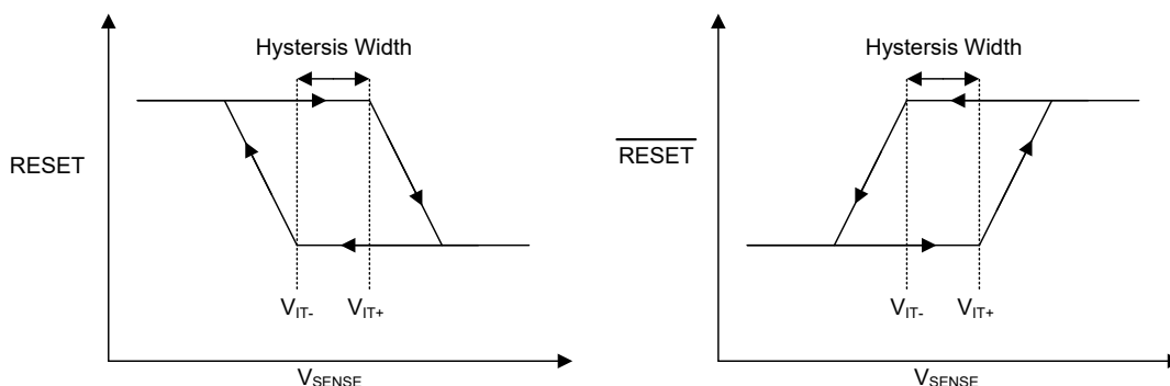
Figure 7-3. Hysteresis Diagram
