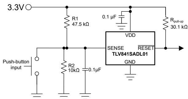
Figure 8-1. Design 1 - Adjustable Voltage Supervisor with Push-Button Functionality Circuit
