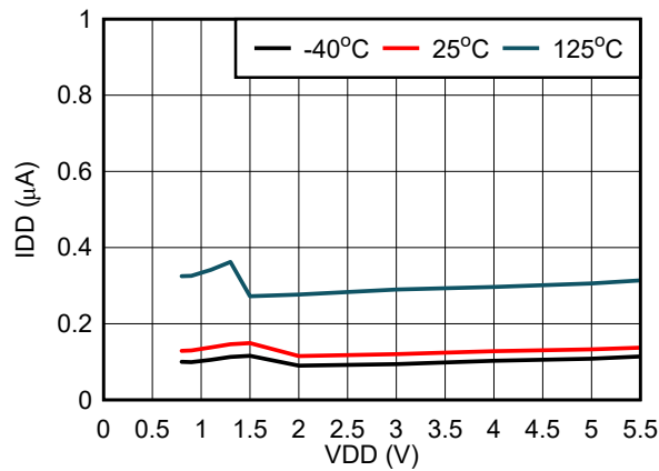
Figure 6-5. Supply Current vs Supply Voltage for TLV841S
