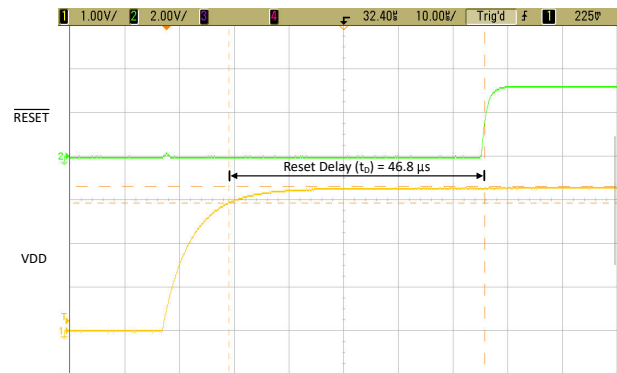
Figure 8-4. TLV841EVM RESET Time Delay ( t_D )
