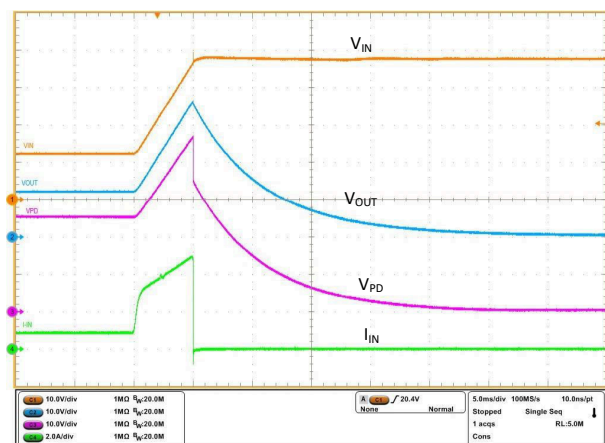
Figure 9-16. Overvoltage Protection
