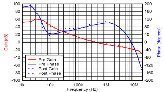
Figure 9-11. Bode Plot: Unit 1 with I_{OUT} = 1 \text{ A}
