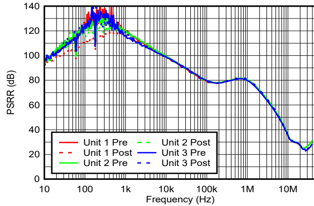
Figure 9-6. PSRR with I_{OUT} = 100 \text{ mA}
