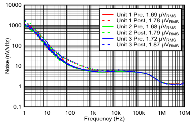
Figure 9-9. Noise Spectral Density with I_{OUT} = 1 \text{ A}
