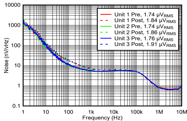
Figure 9-8. Noise Spectral Density with I_{OUT} = 100 \text{ mA}
