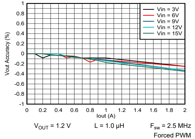
Figure 9-20. Output Voltage vs Output Current
