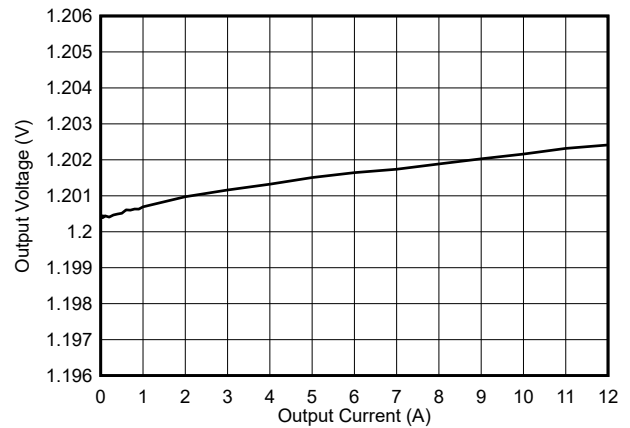
Figure 8-3. Load Regulation
