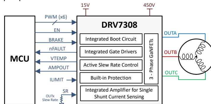
Simplified Schematic
