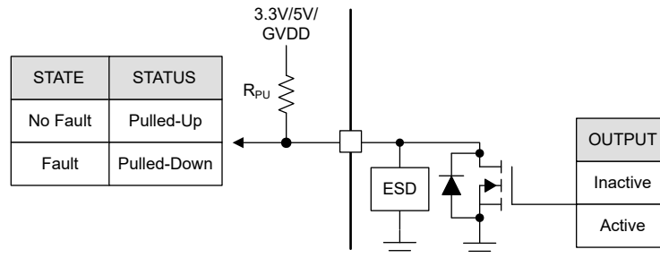
Figure 12-4. Open-Drain Pin Structure
