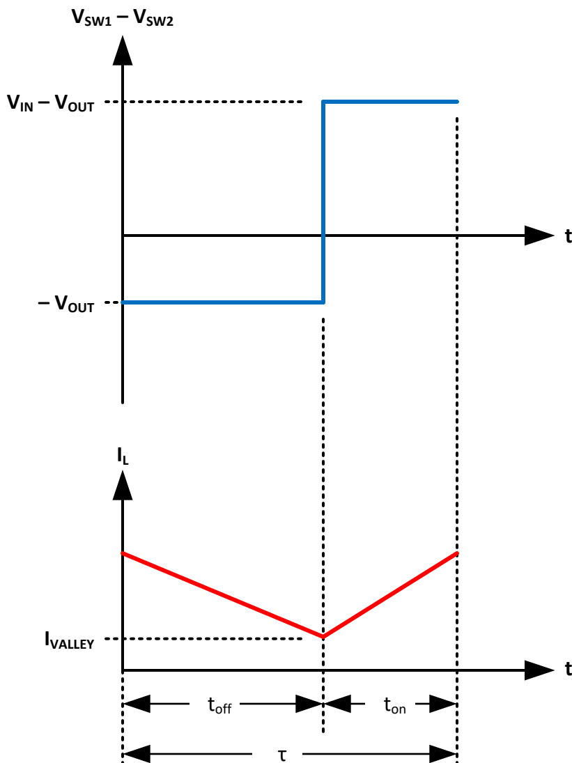
Figure 8-9. Buck State
