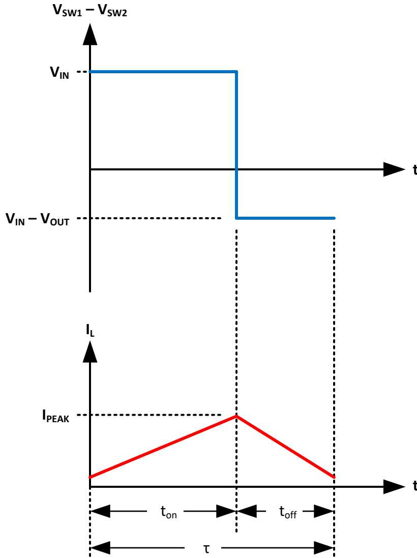
Figure 8-12. Boost State
