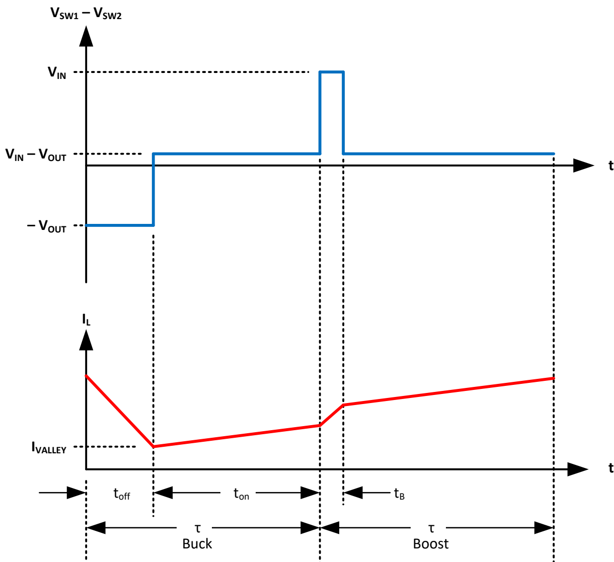
Figure 8-10. Buck Transition
