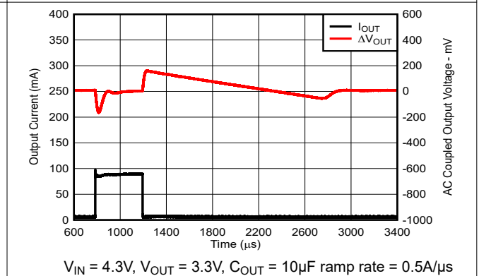
Figure 5-16. I_{OUT} Transient From 1mA to 80mA
