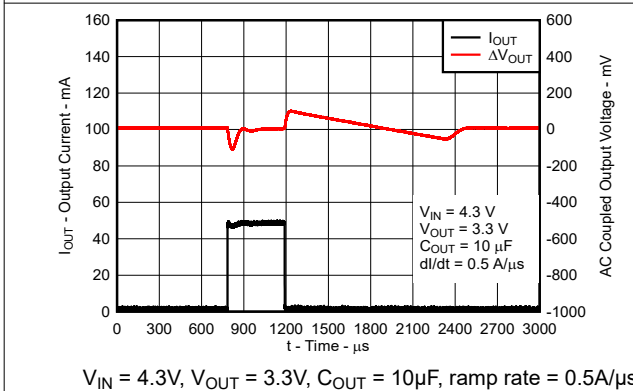
Figure 5-15. I_{OUT} Transient From 1mA to 50mA
