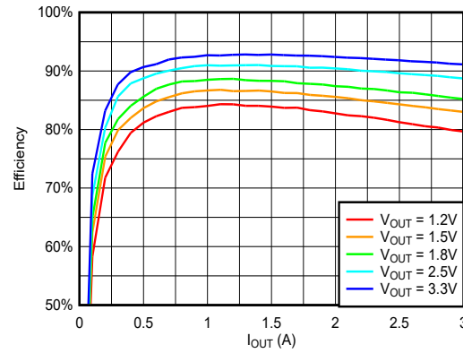
Figure 6-38. Efficiency vs Load at VIN = 7V, Across VOUT at fsw = 500kHz for Channel # 1 at 25°C
