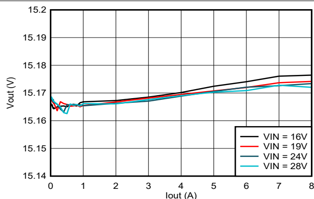
Figure 7-3. Load Regulation
