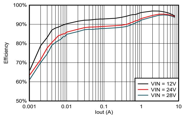
Figure 5-11. Efficiency, Vout = 5V
