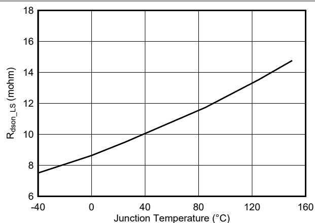
Figure 5-4. Low-Side R_{DS(on)} vs Temperature
