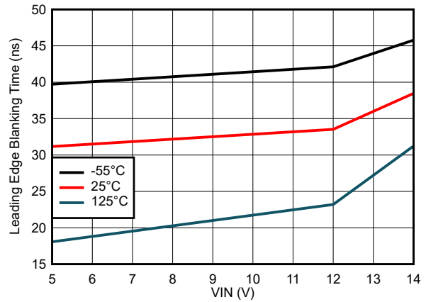
Figure 6-38. Leading Edge Blanking Time vs Input Voltage
