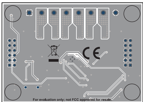
Figure 4-5. Bottom View
