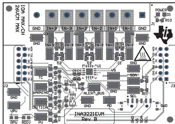
Figure 4-3. Top View
