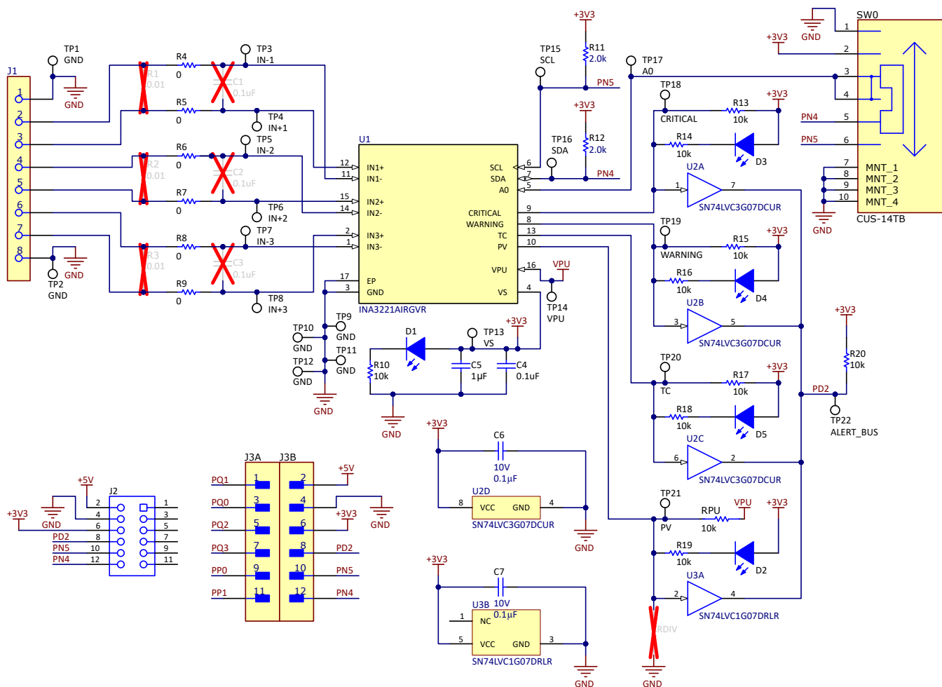
Figure 4-1. Schematic Circuitry
