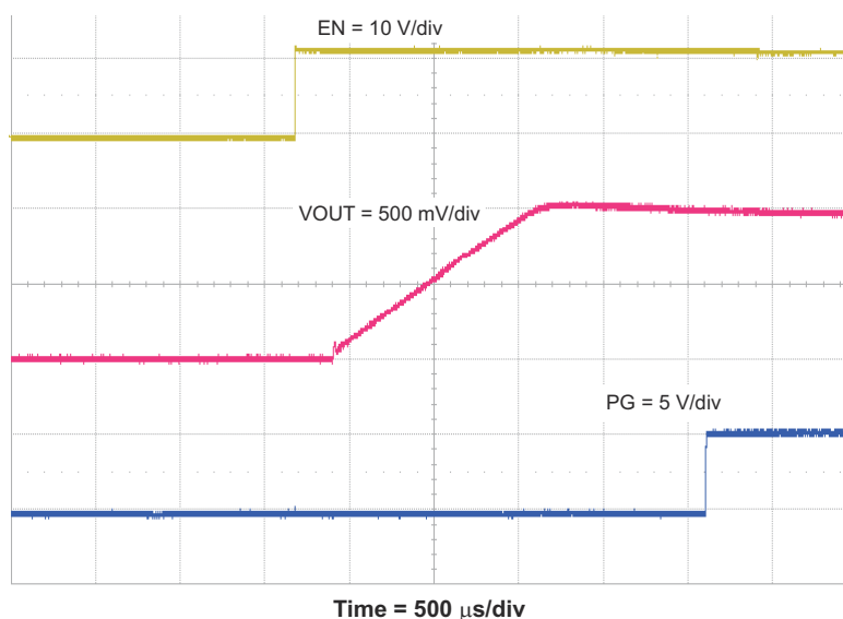
Figure 2-7. TPS54326EVM-540 Start-Up
