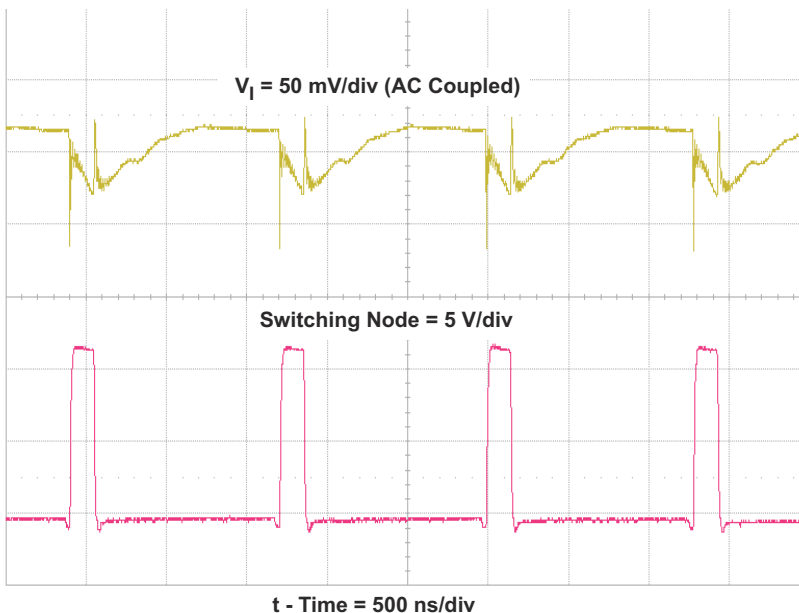
Figure 2-6. TPS54326EVM-540 Input Voltage Ripple
