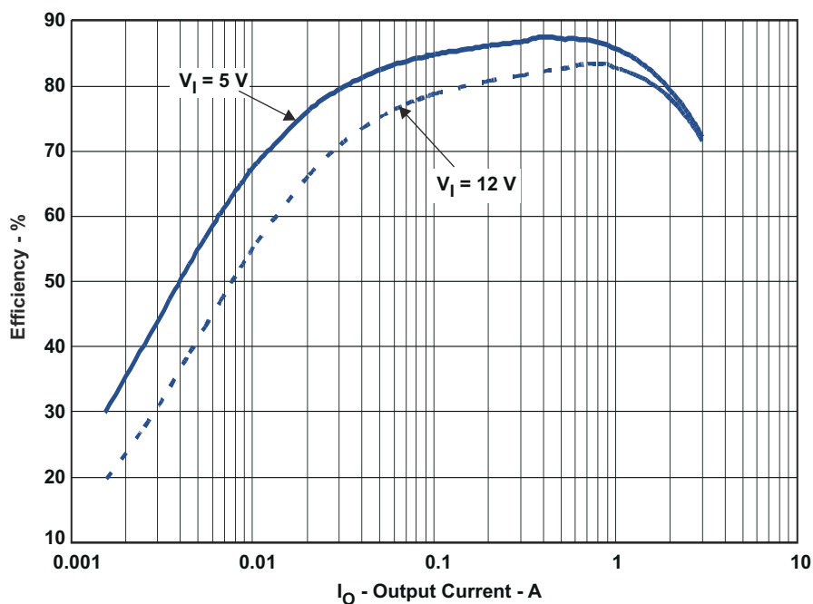
Figure 2-1. TPS54326EVM-540 Efficiency
