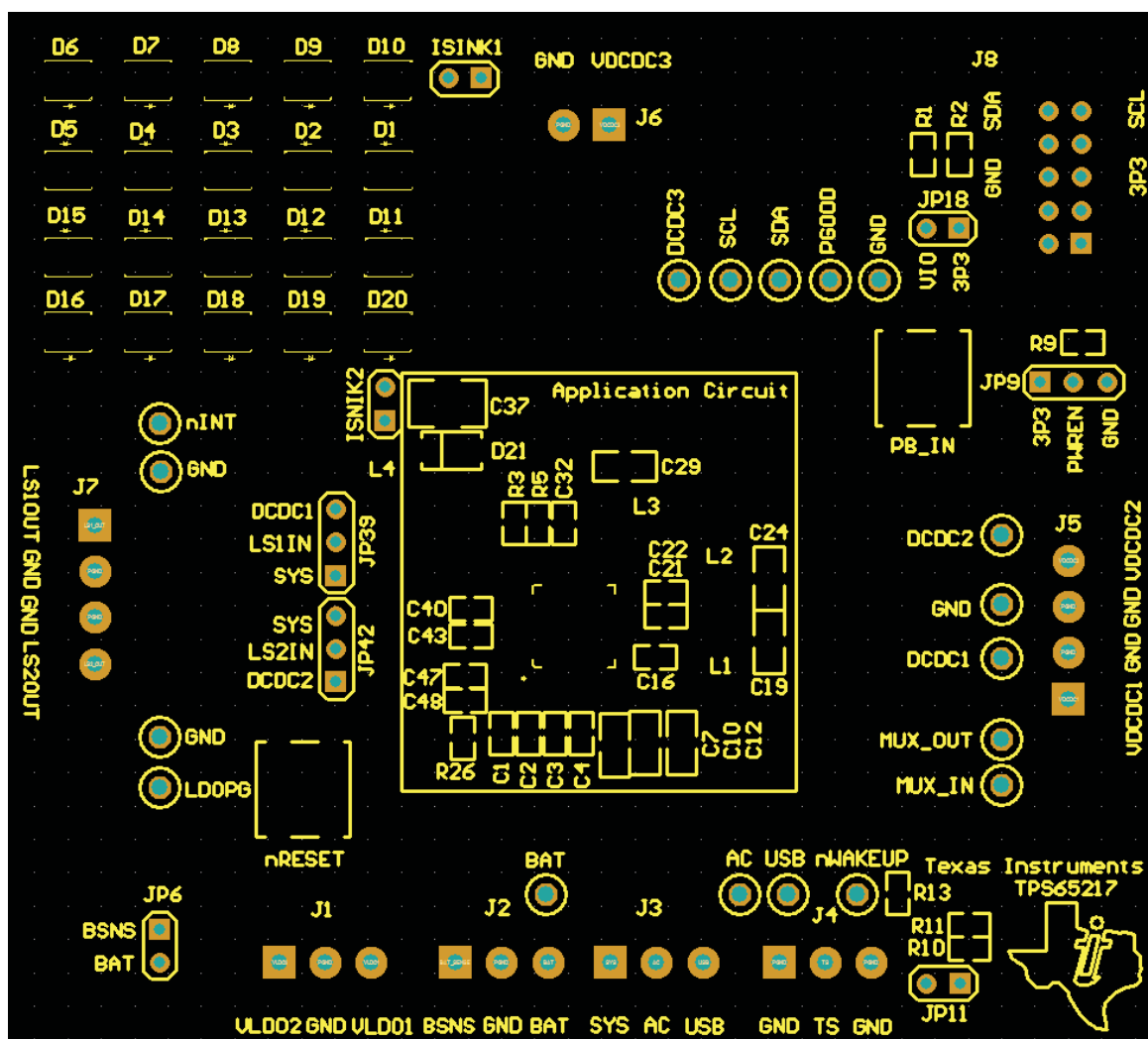
Figure 4. Layout - Silkscreen
