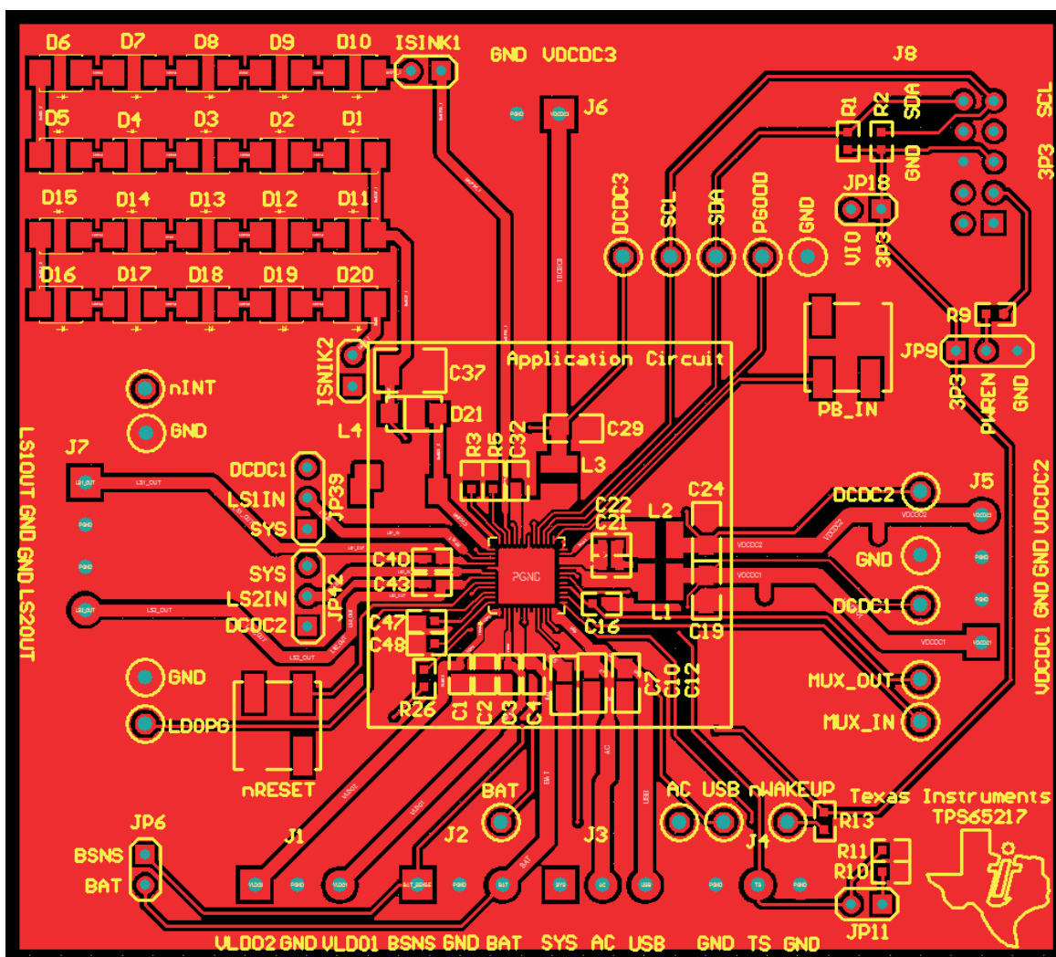
Figure 5. Layout - Top Layer Silkscreen
