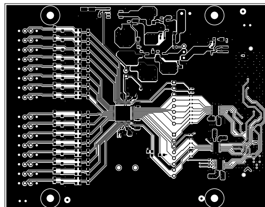
Figure 4-7. Top Layer
