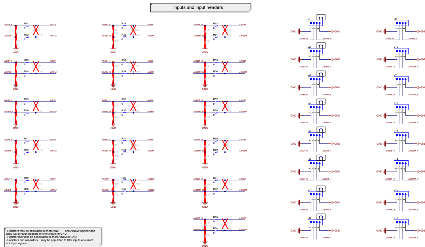
Figure 4-1. Inputs Schematic
