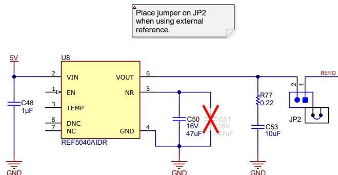
Figure 2-3. REF5040
