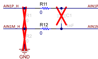
Figure 2-2. Current Sense Input Channel
