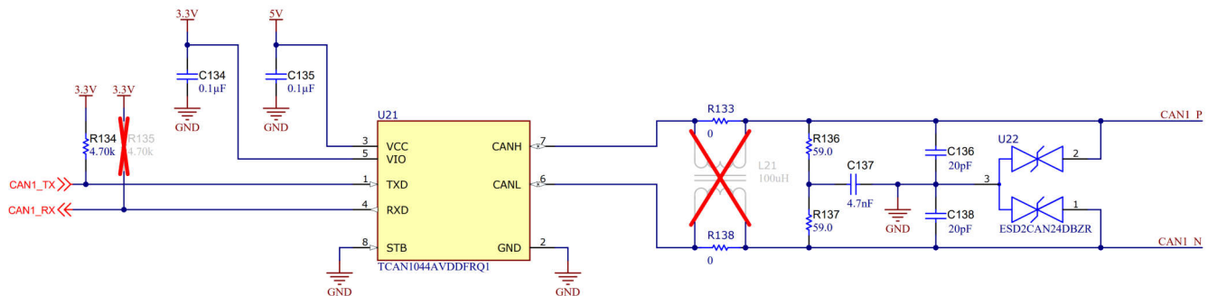
Figure 2-4. CAN Circuit
