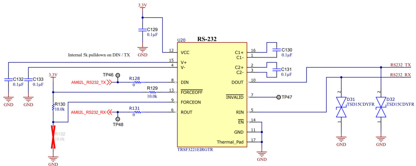
Figure 2-3. RS-232 Circuit
