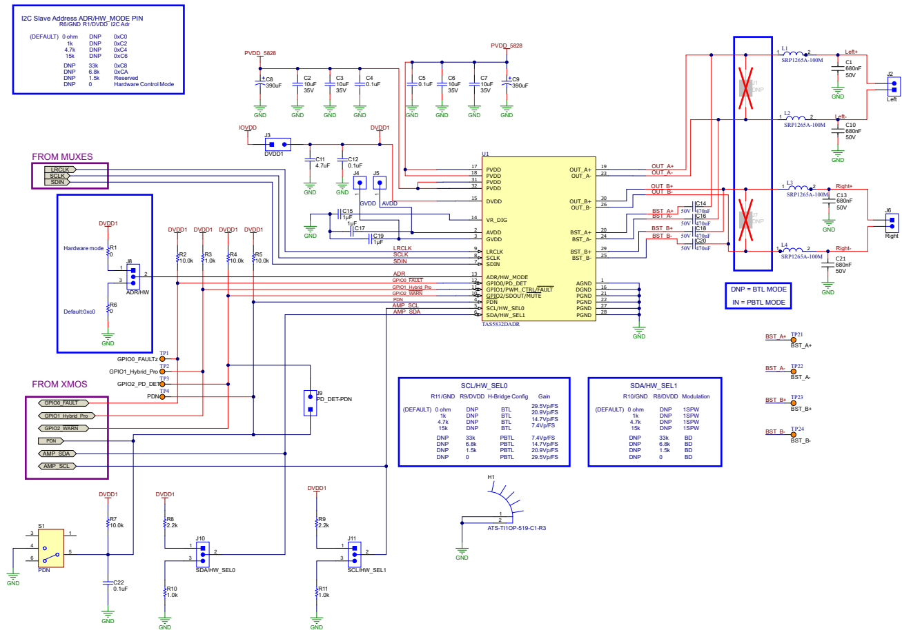
Figure 3-1. TAS5832EVM Schematic (1 of 5)
