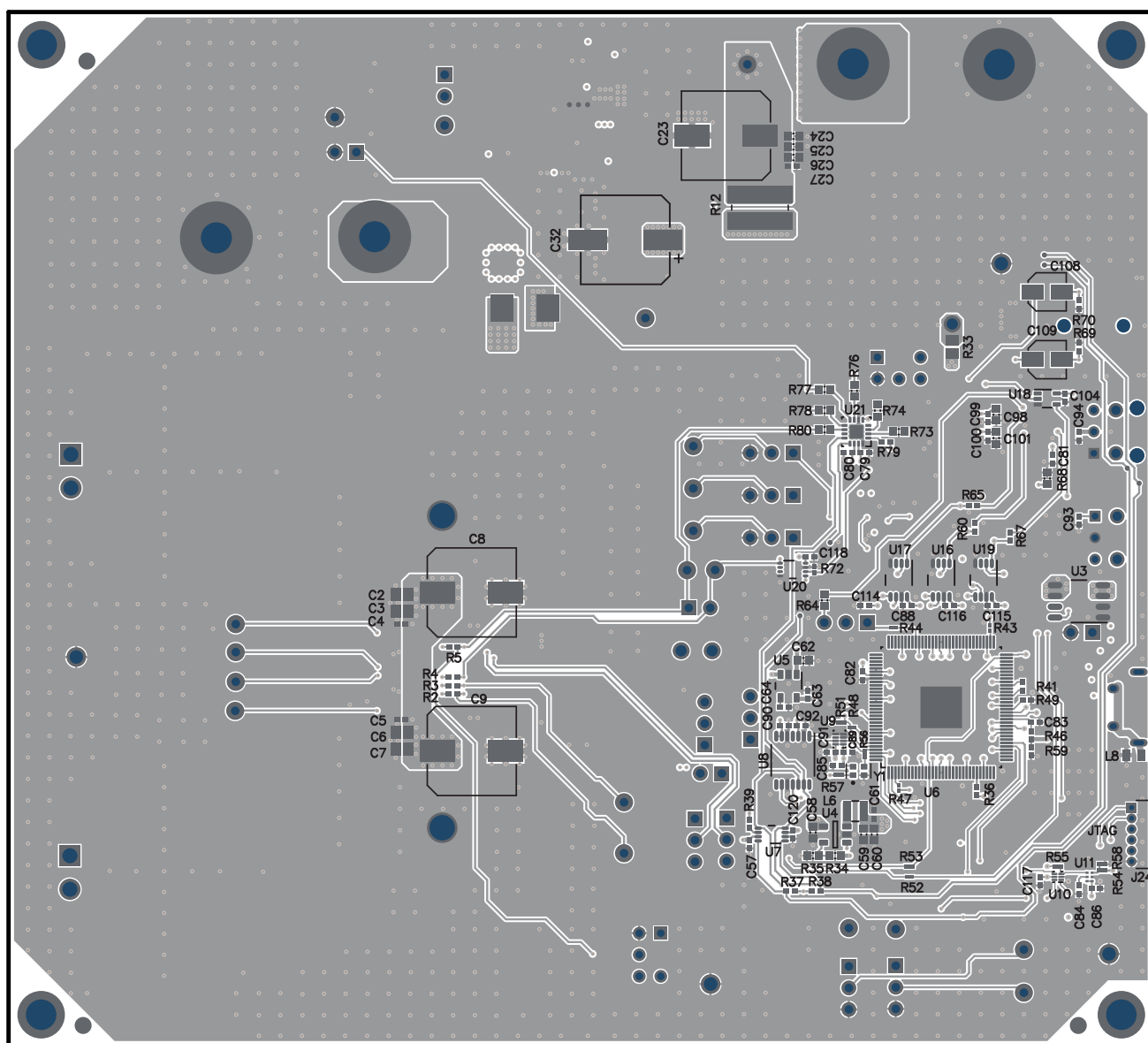
Figure 3-7. TAS5832EVM Bottom Overlay
