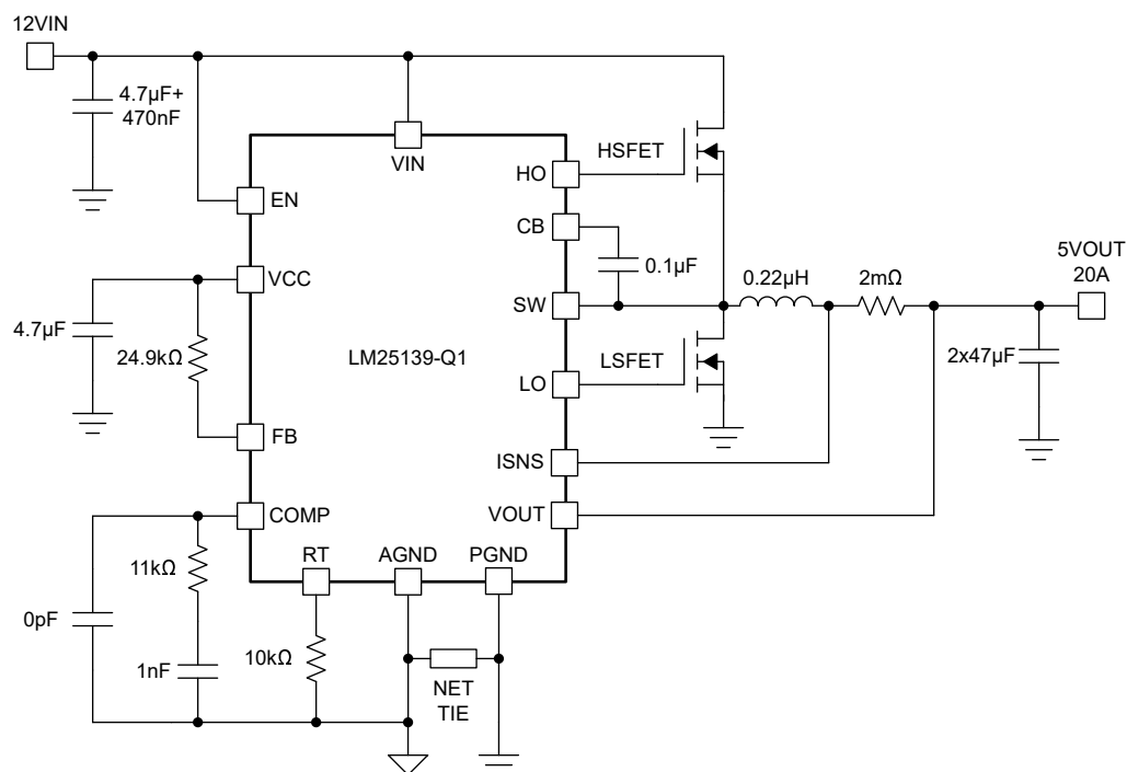
Figure 3-7. 2.2MHz Schematic, Simplified
