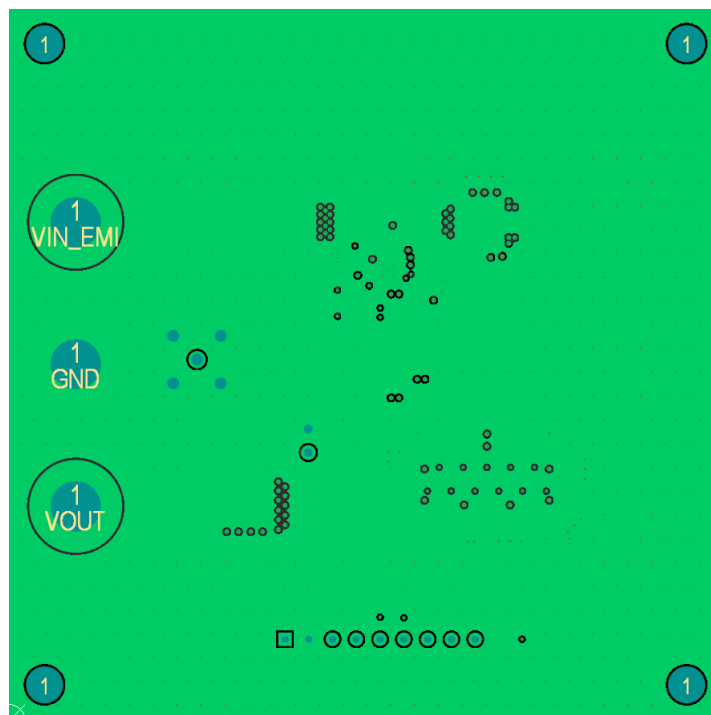
Figure 4-7. Layer 4 Copper (Top View)
