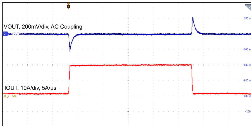
Figure 3-6. 1MHz Schematic Load Transient Response, V_{IN} = 12V , FPWM, 0A to 20A, 5A/µs
