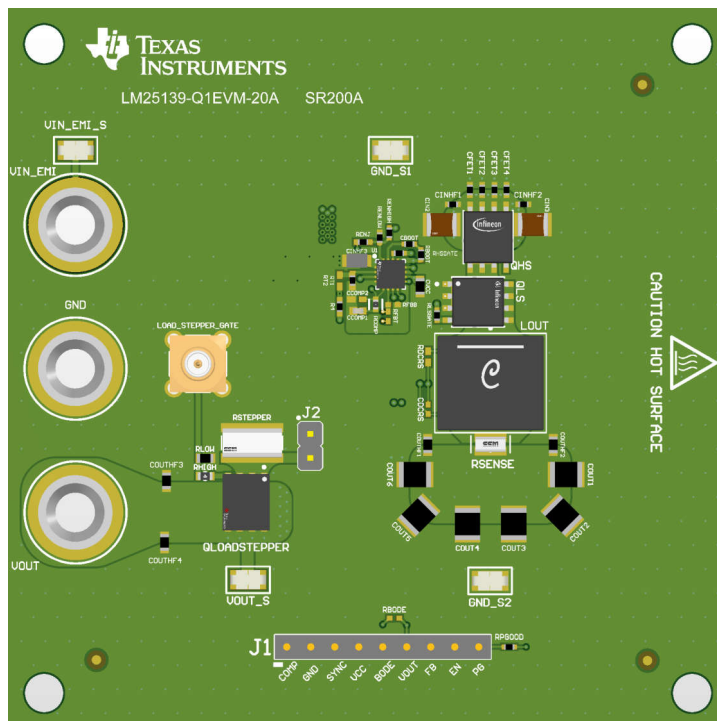
Figure 4-2. PCB (Top View)
