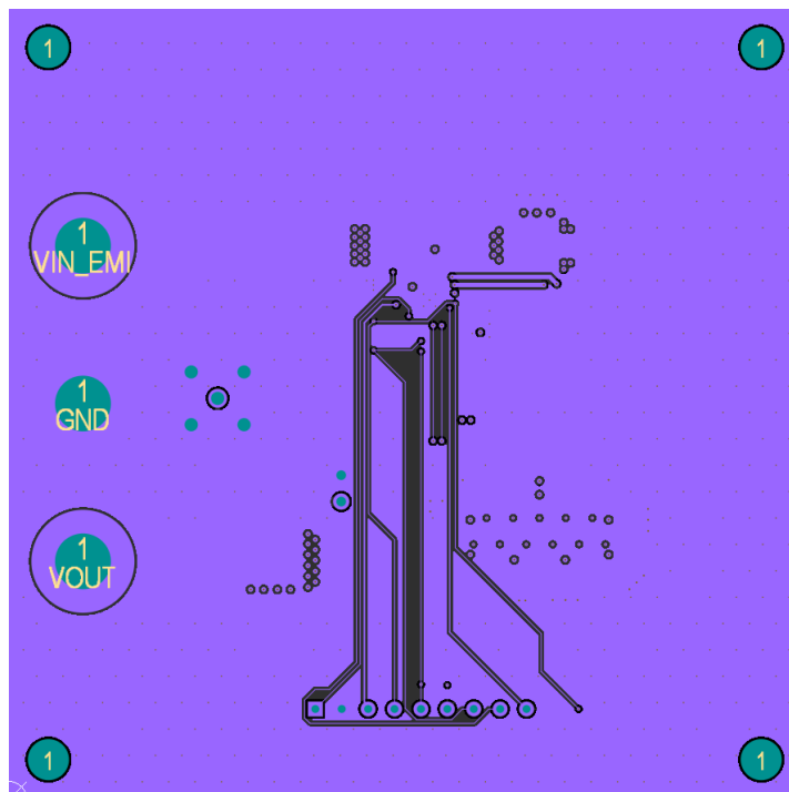
Figure 4-8. Layer 5 Copper (Top View)
