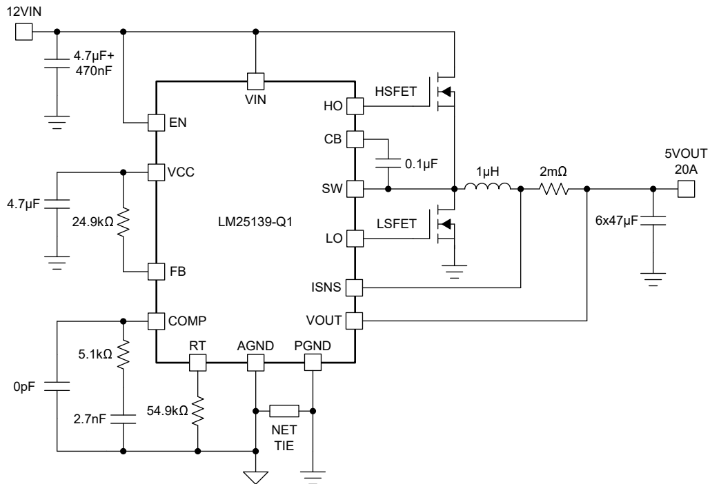
Figure 3-3. Default Schematic, Simplified
