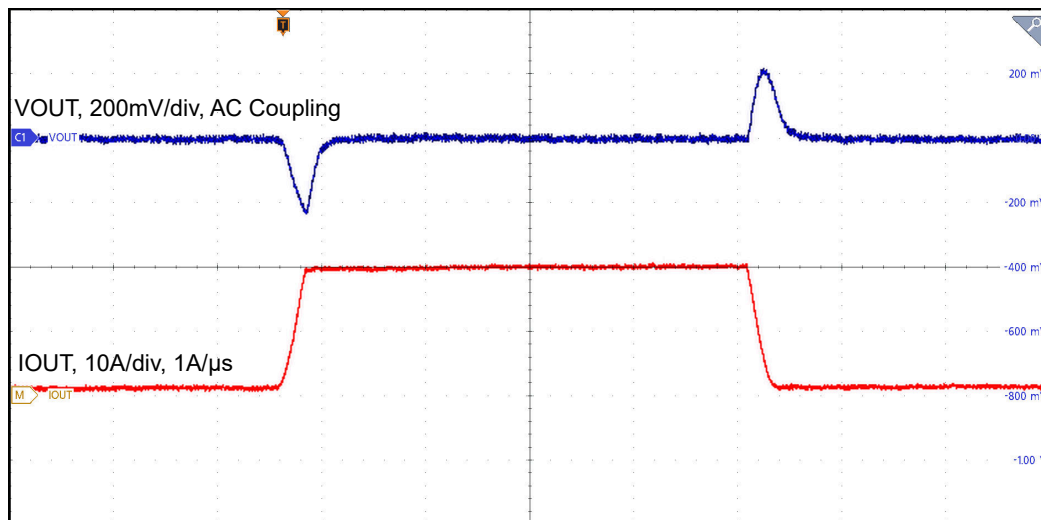
Figure 3-4. Load Transient Response, V_{IN} = 12V , FPWM, 0A to 20A, 1A/µs
