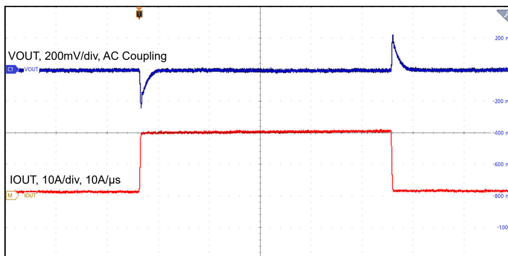
Figure 3-8. 2.2MHz Schematic Load Transient Response, V_{IN} = 12V , FPWM, 0A to 20A, 10A/µs
