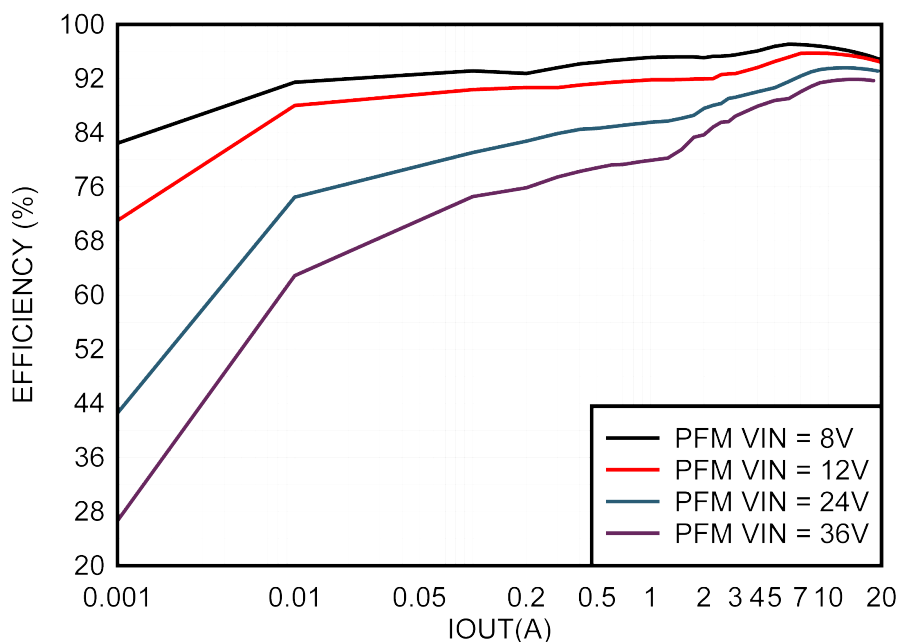
Figure 3-2. Efficiency, V_{OUT} = 5V , PFM (Log Scale)
