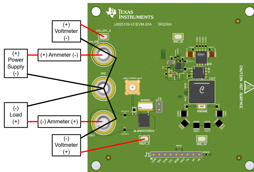
Figure 2-1. EVM Test Setup
