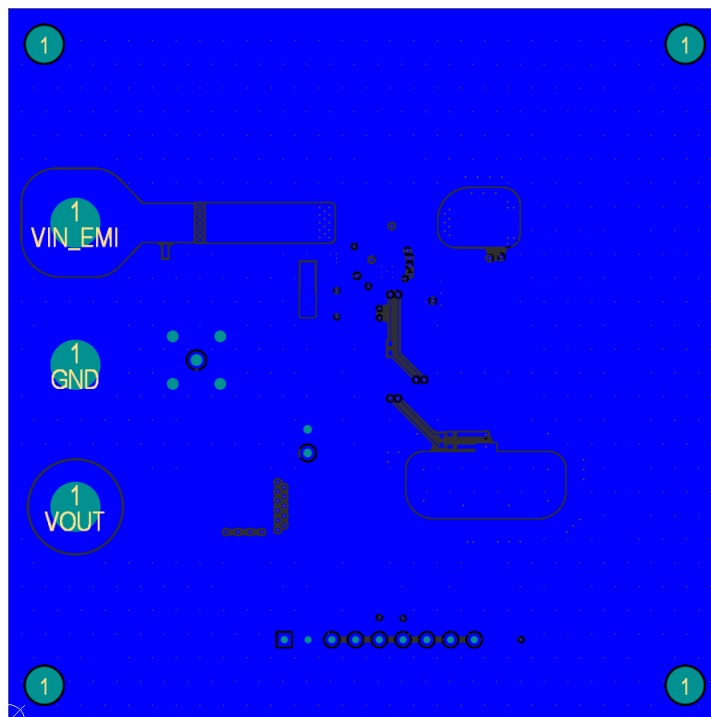
Figure 4-9. Bottom Copper (Top View)
