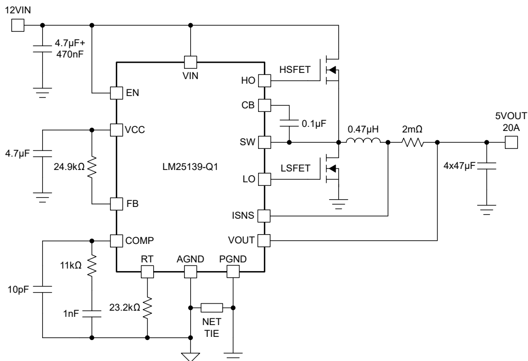
Figure 3-5. 1MHz Schematic, Simplified
