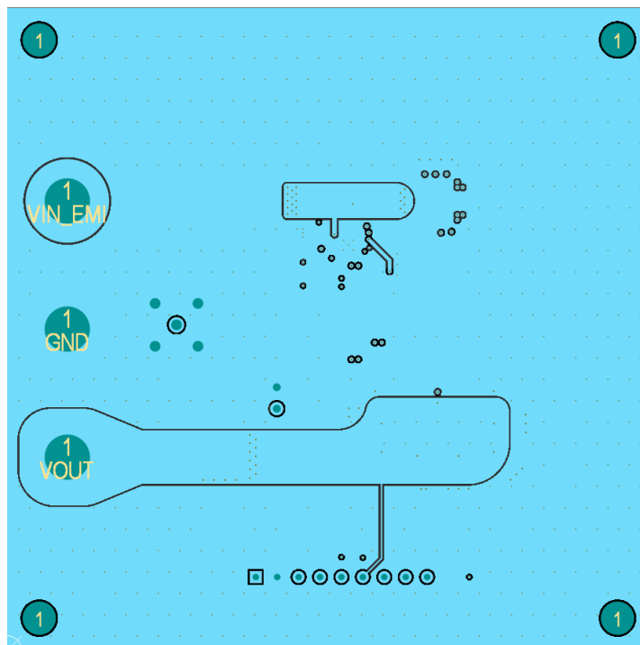
Figure 4-6. Layer 3 Copper (Top View)
