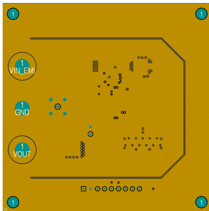
Figure 4-5. Layer 2 Copper (Top View)
