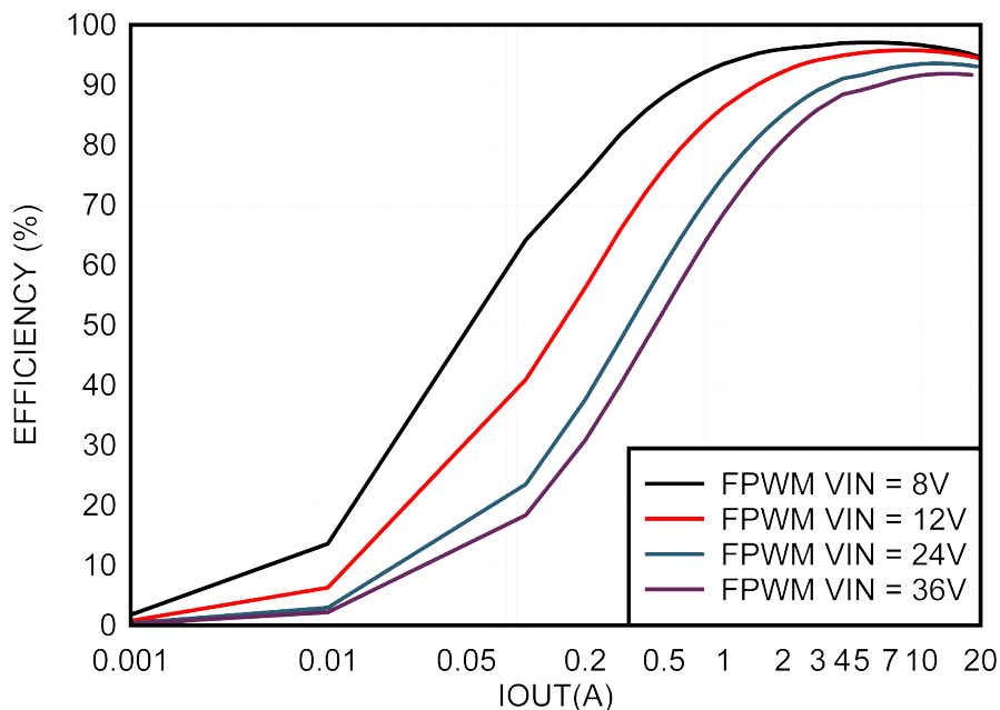
Figure 3-1. Efficiency, V_{OUT} = 5V , FPWM (Log scale)
