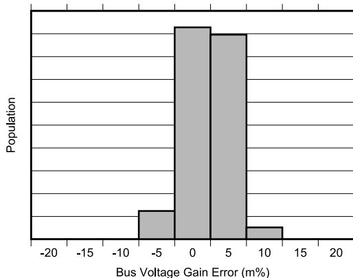
Figure 5-12. Bus Input Gain Error Production Distribution
