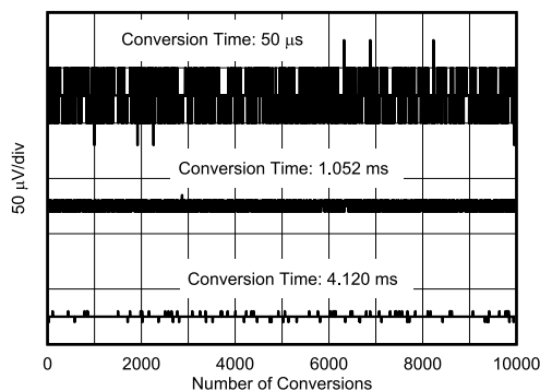
Figure 6-4. Noise vs. Conversion Time (Averaging = 1)
