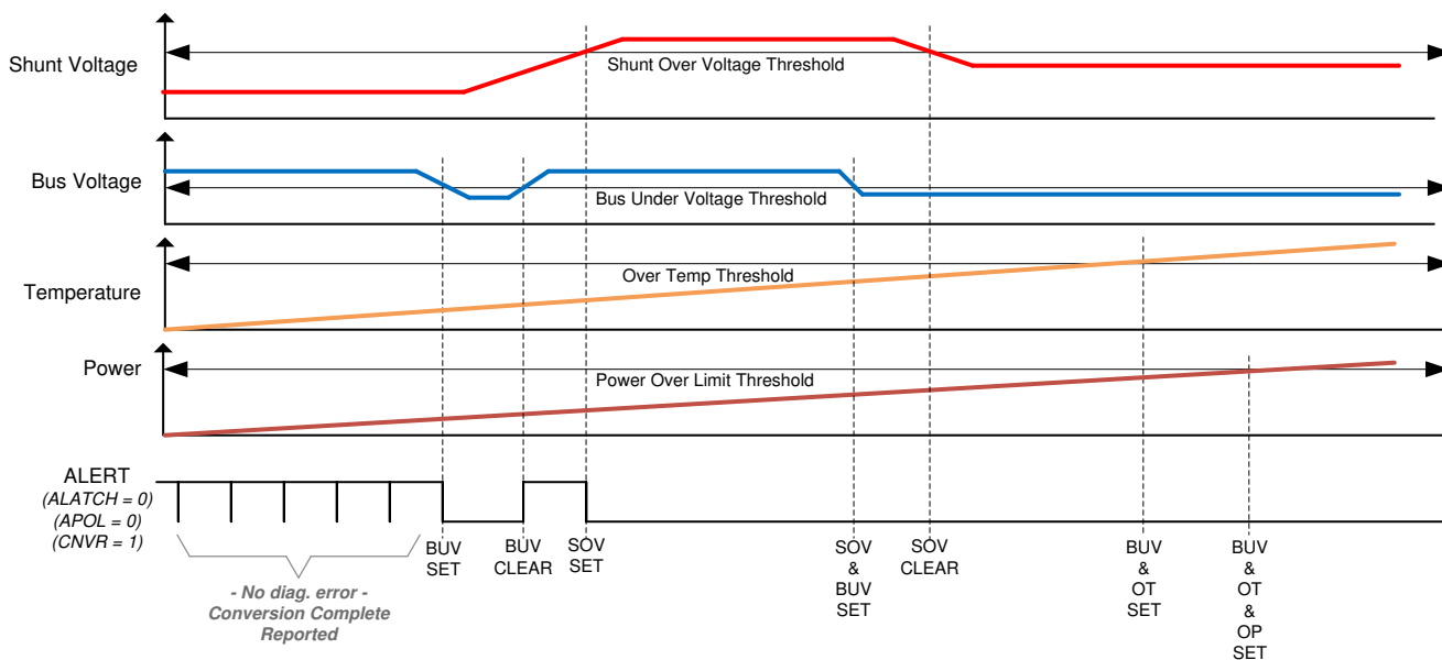
Figure 6-6. Multi-Alert Configuration
