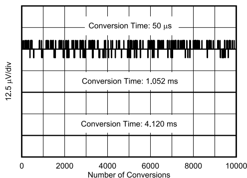
Figure 6-5. Noise vs. Conversion Time (Averaging = 128)
