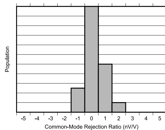
Figure 5-5. Common-Mode Rejection Ratio Production Distribution
