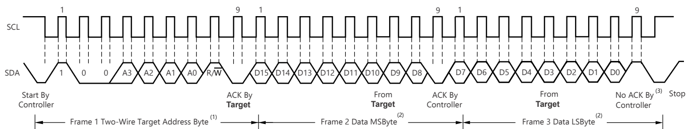
Figure 6-7. Timing Diagram for Write Word Format
