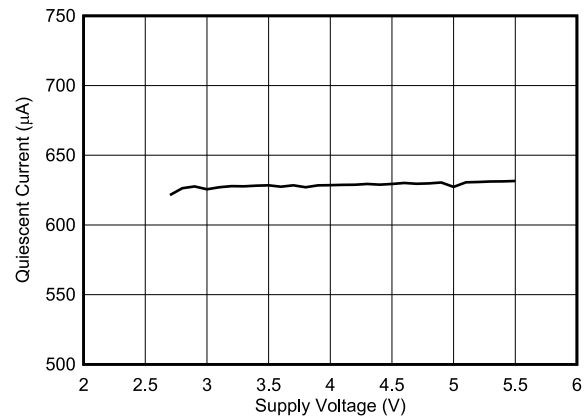
Figure 5-19. Active I_Q vs Supply Voltage
