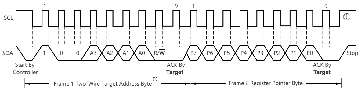
Figure 6-9. Typical Register Pointer Set
