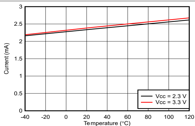
Figure 5-3. Active Mode ICC vs Temperature
