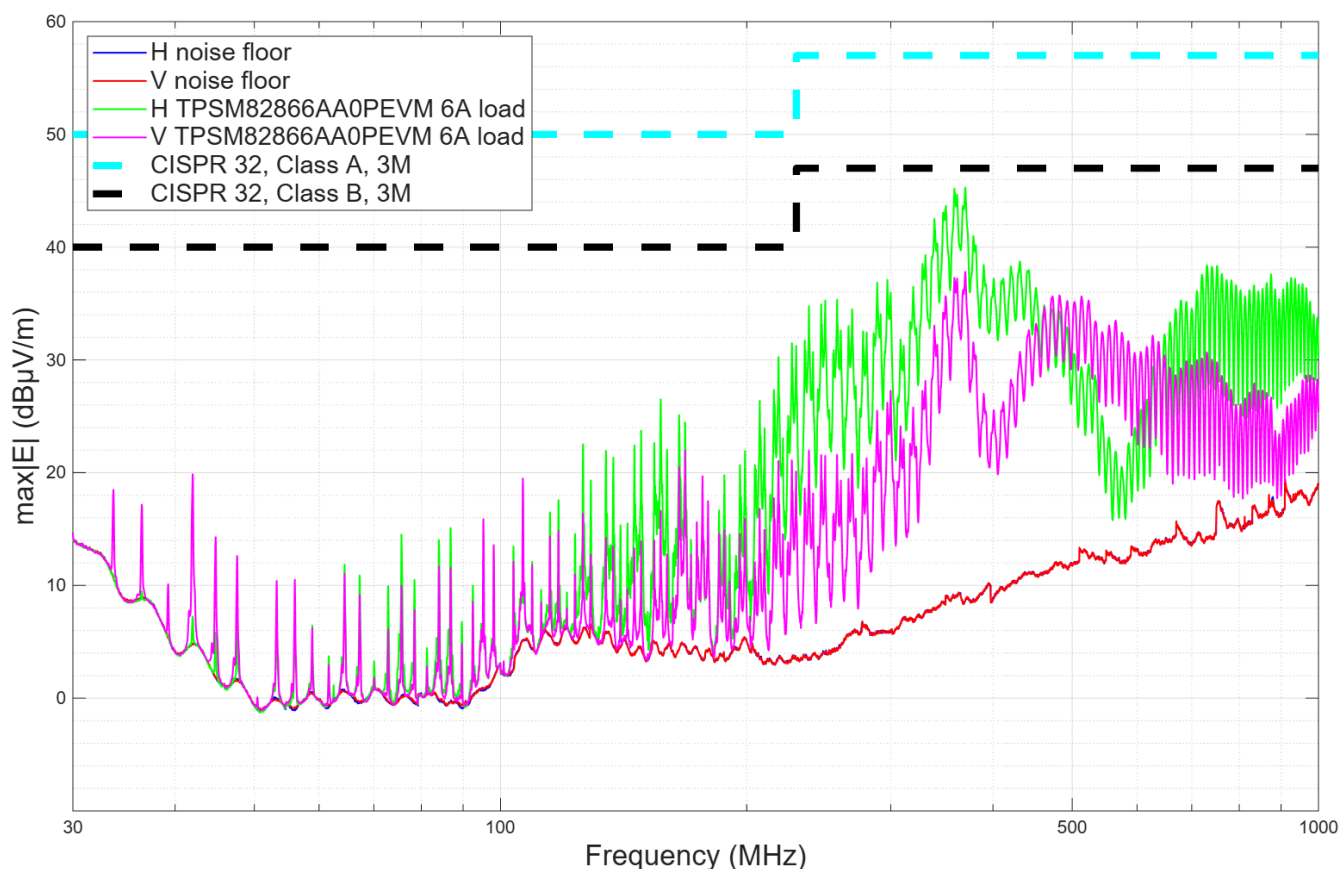
Figure 4. Radiated EMI performance of a 6A power module with MagPack technology from 30MHz to 1GHz, demonstrating compliance with CISPR32 Class A and Class B limits
