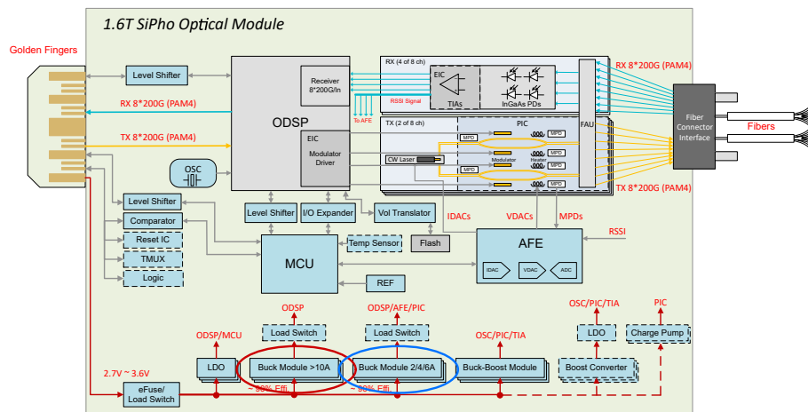
Figure 1. System block diagram of a 1.6Tbps optical module
