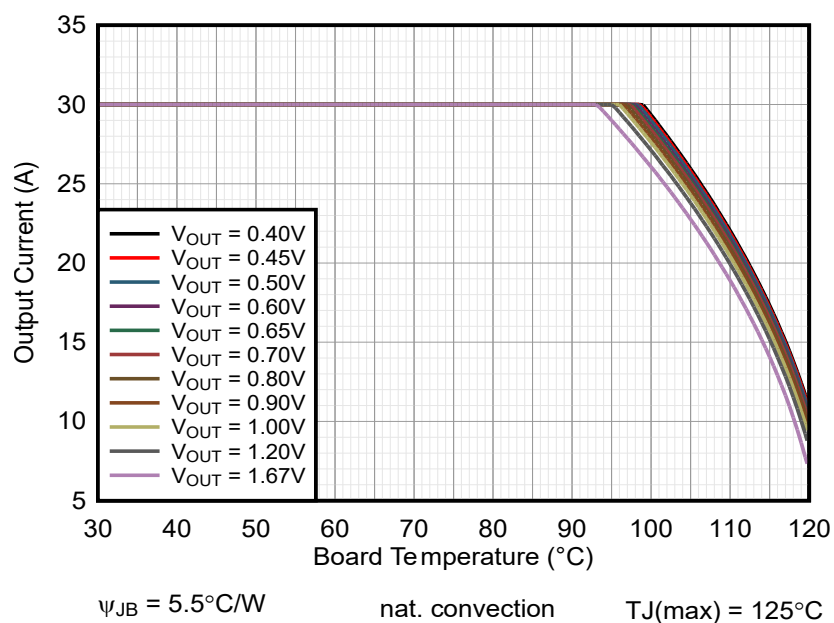
Figure 3. SOA curve of the TPSM8287B30 power module at V_{IN} = 5.0\text{V}
