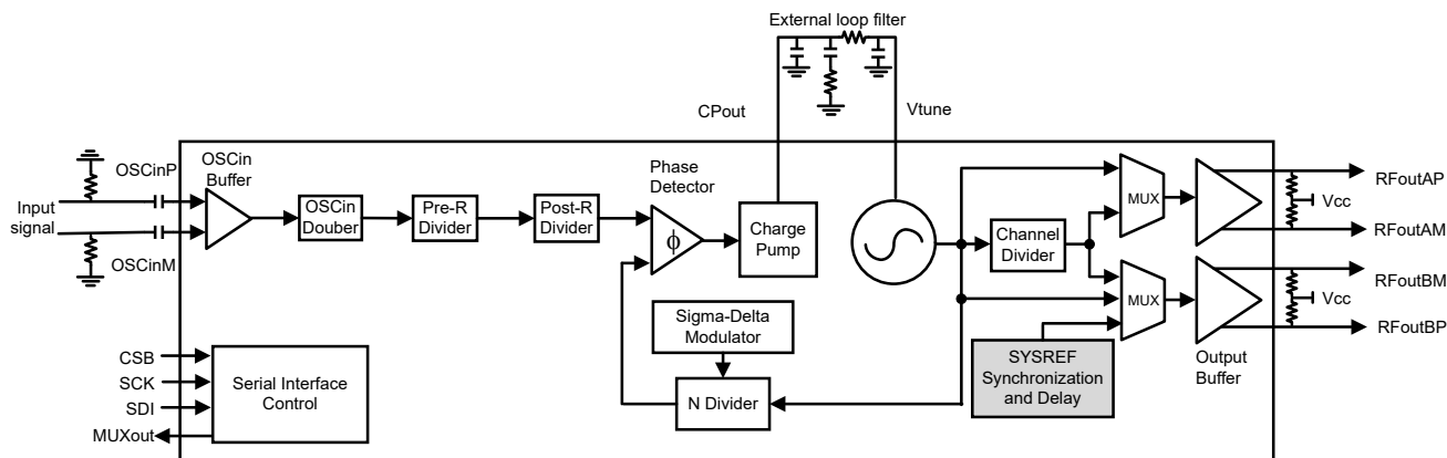
Figure 3-1. Simplified Schematic
