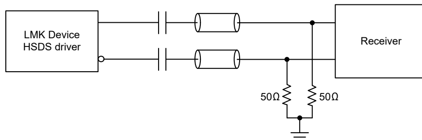
Figure 7-29. AC-Coupled HSDS Output Termination Method 2
