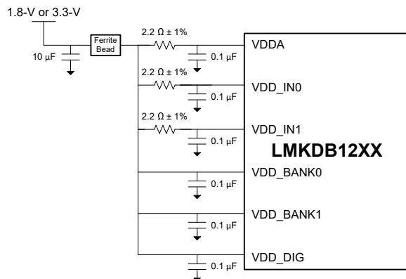
Figure 10-5. Power Supply Recommendation for LMKDB12XX MUX
