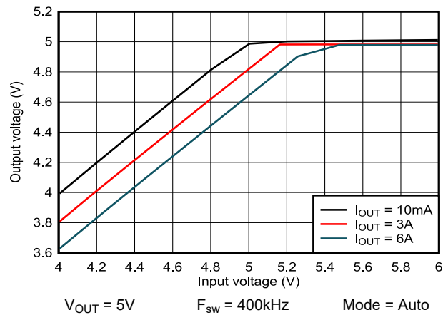
Figure 8-19. Dropout Curve
