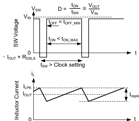
Figure 7-11. Dropout Waveforms
