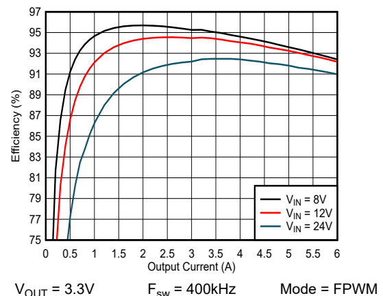
Figure 8-3. Efficiency - FPWM Mode
