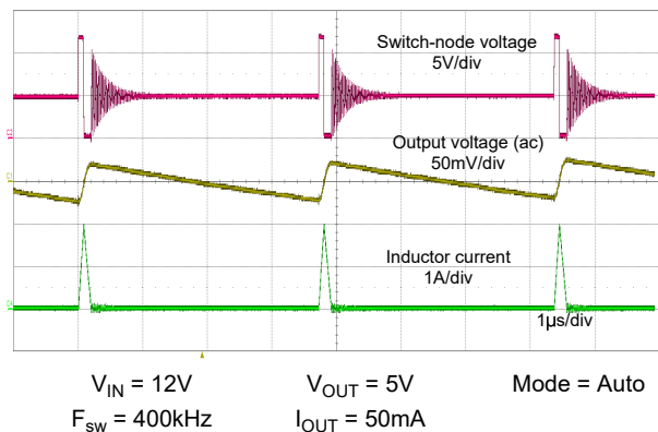
Figure 8-28. Steady-State Switching Waveform and Output Voltage Ripple
