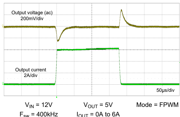
Figure 8-25. Load Transient
