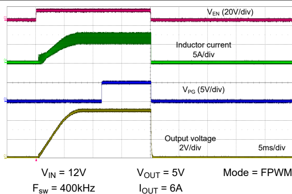
Figure 8-31. Enable Start-Up and Shutdown With 6A Load
