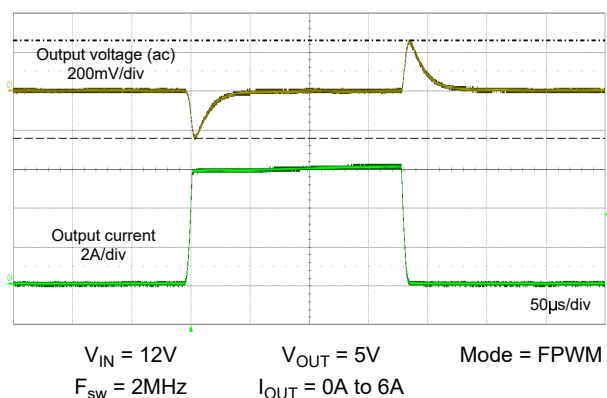
Figure 8-27. Load Transient
