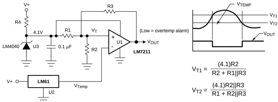
Figure 15. Centigrade Thermostat
