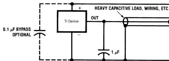
Figure 8-1. No Decoupling Required for Capacitive Load
