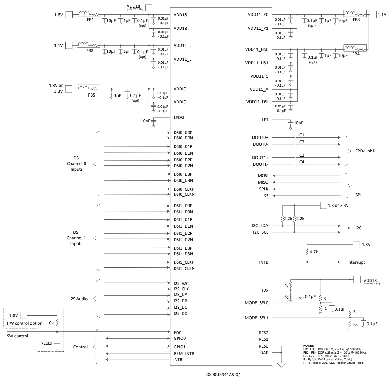
Figure 9-1. Typical Connection Diagram - STP
