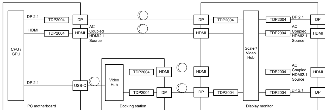
Figure 7-1. Typical Application
