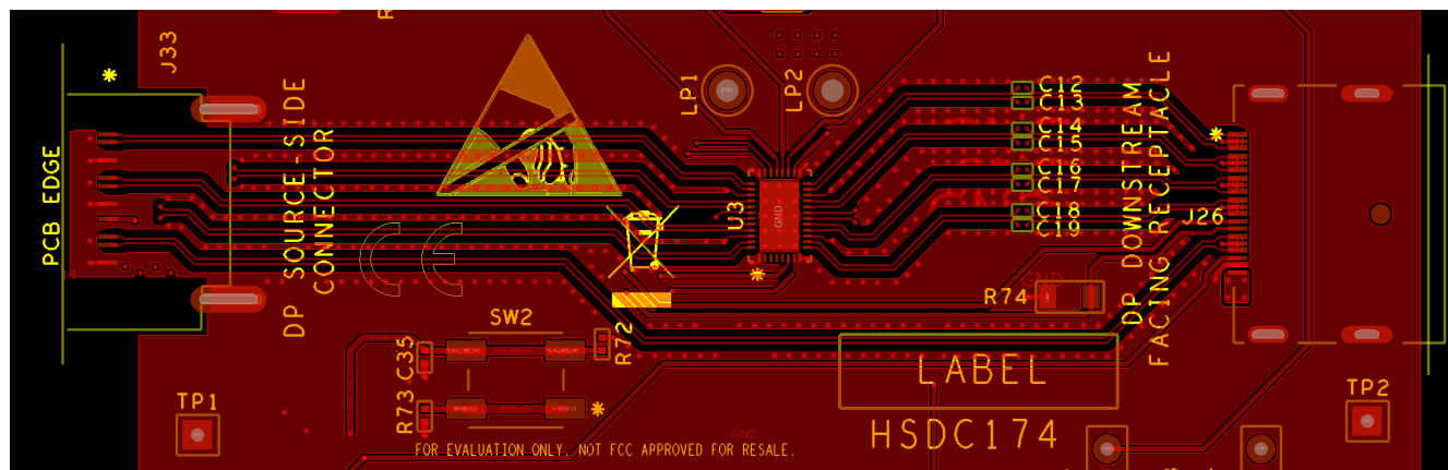
Figure 7-8. TDP2004 Layout Example – Sub-Section of TI Evaluation Board with DP Connectors
