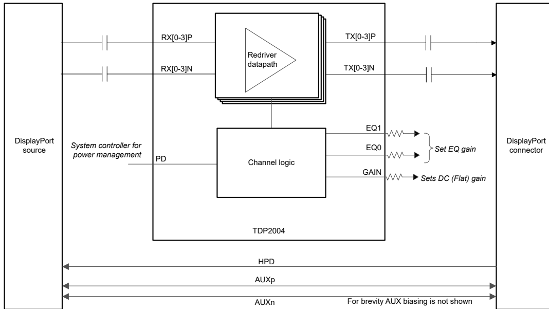
Figure 7-2. Simplified Schematic for DP 2.1 Signal Conditioning in a Source Application such as PC Motherboard
