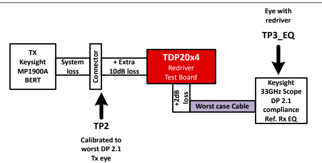
Figure 7-5. A Typical 20Gbps (UHBR20) DP 2.1 Tx Compliance Channel Setup with Redriver
