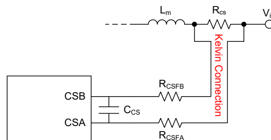
Figure 7-4. Current Sense Filter
