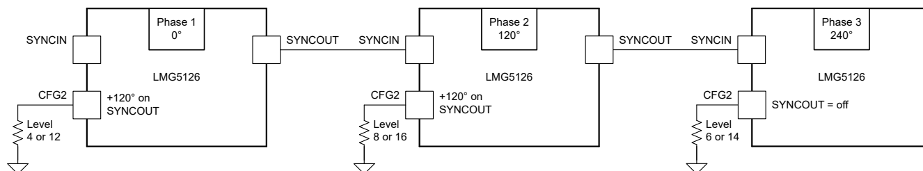
Figure 6-6. 3-Device Configuration
