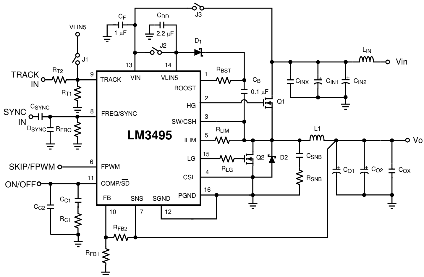
Figure 10-1. Circuit Schematic
