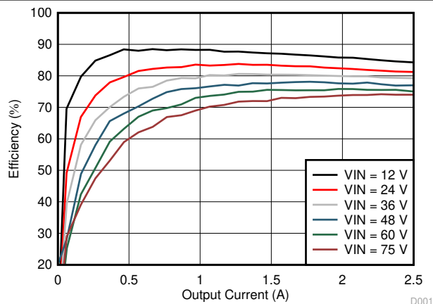
Figure 7-9. Typical Efficiency vs Input Voltage and Output Current, 5V Output
