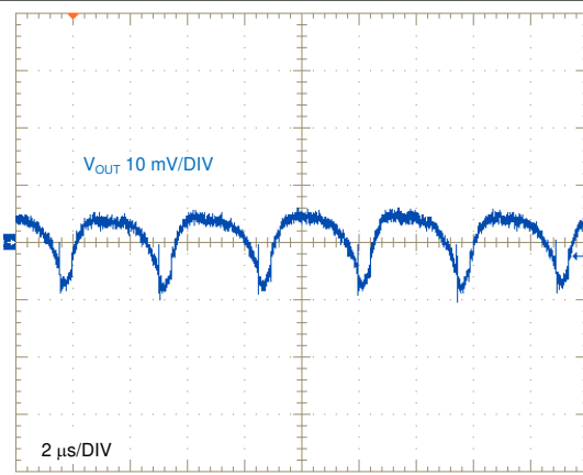
Figure 7-10. Output Voltage Ripple, 2.5A Load
